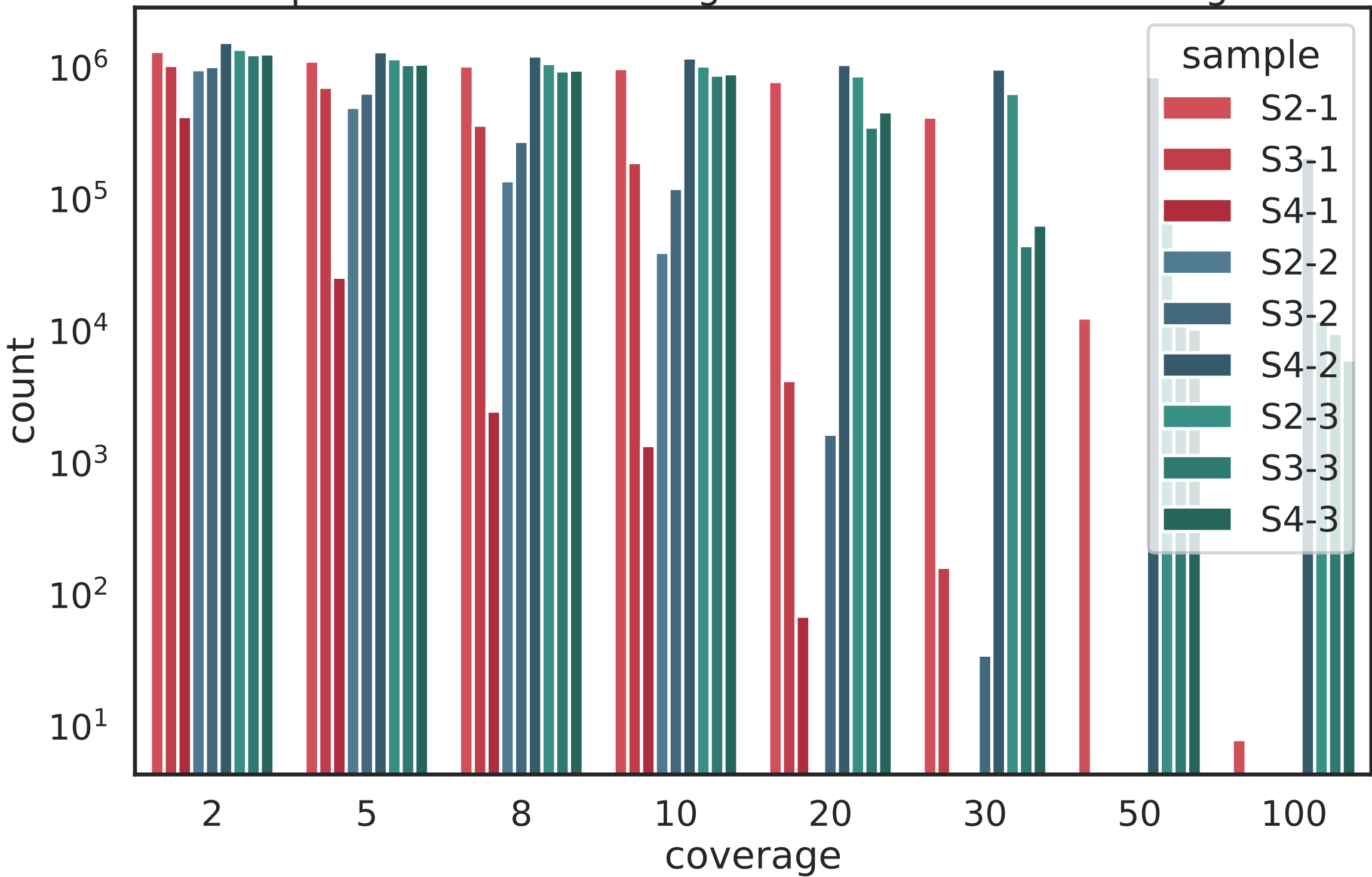
Number of positions with coverage above threshold in Pelagibacter
