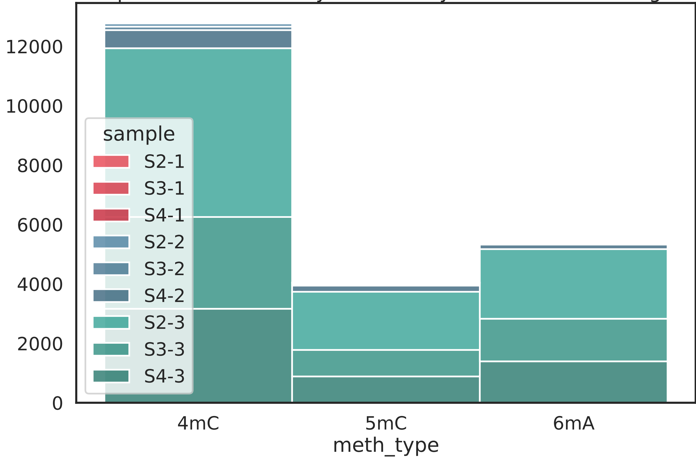
Number of positions 95% methylated in only 1 treatment in Pelagibac
