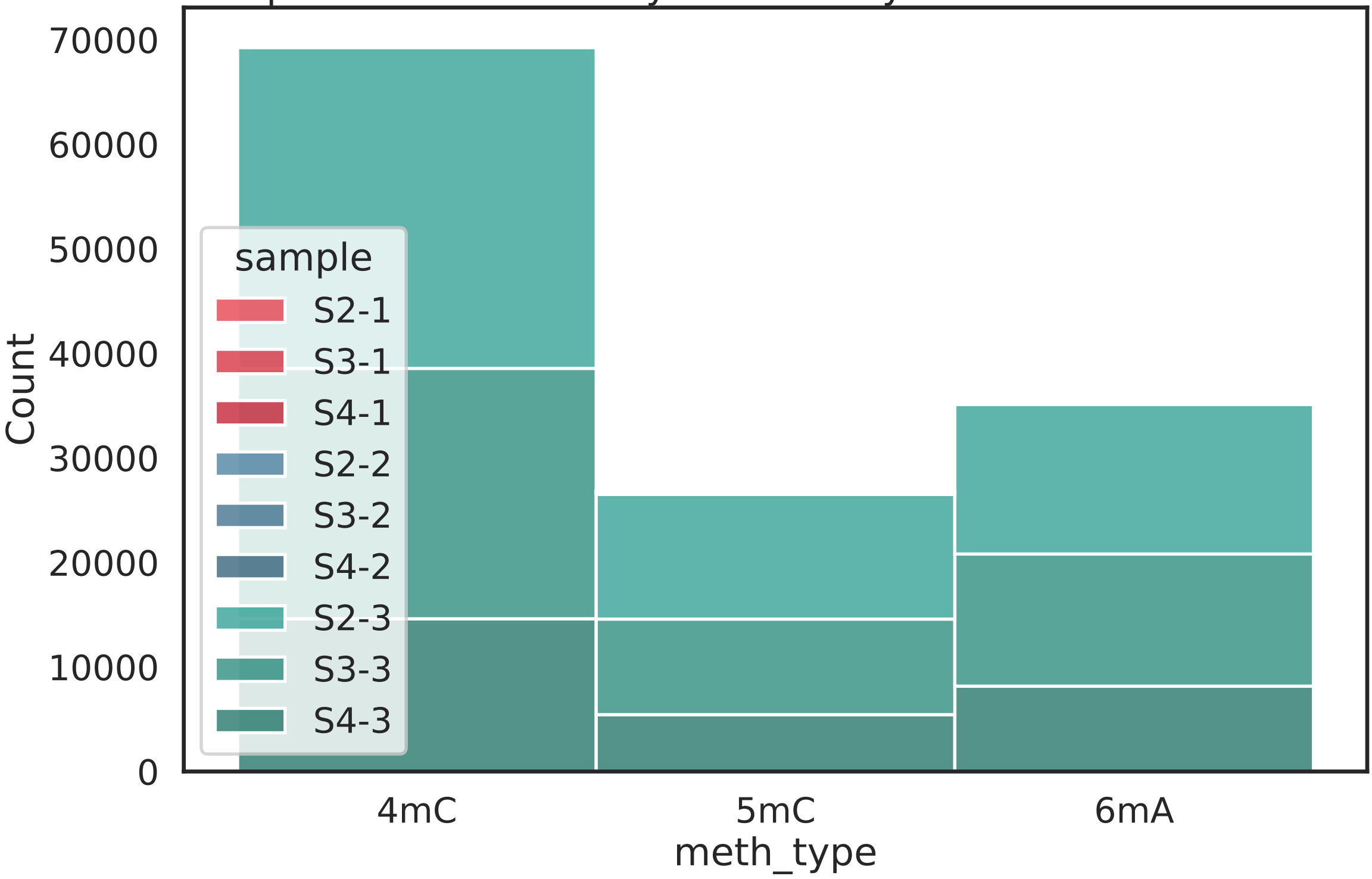
Number of positions 95% methylated in only 1 treatment in Polaribac
