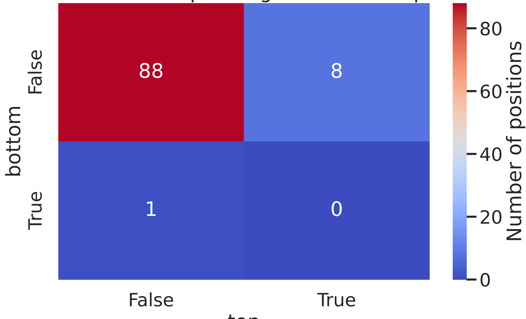
Transition map in Cognaticolwellia sp.
