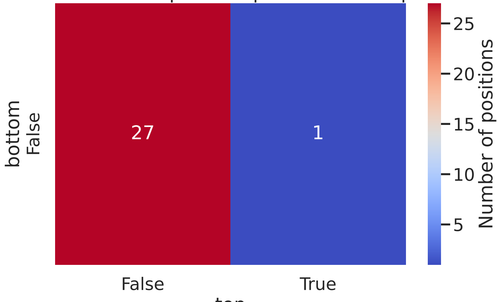
Transition map in Halopseudomonas sp.
