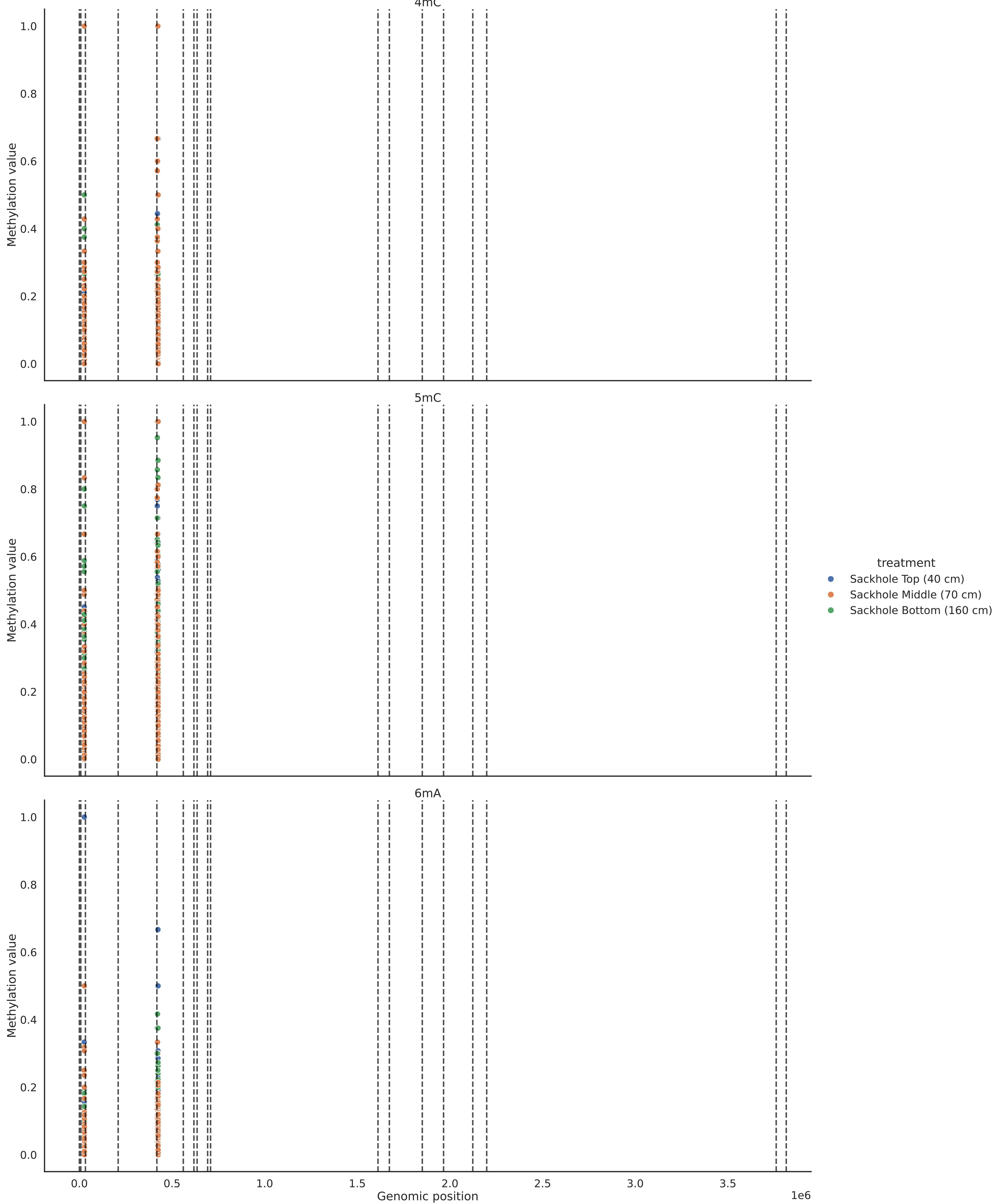
Methylation value across genome of common positions in Psychromonas sp. coverage 8
