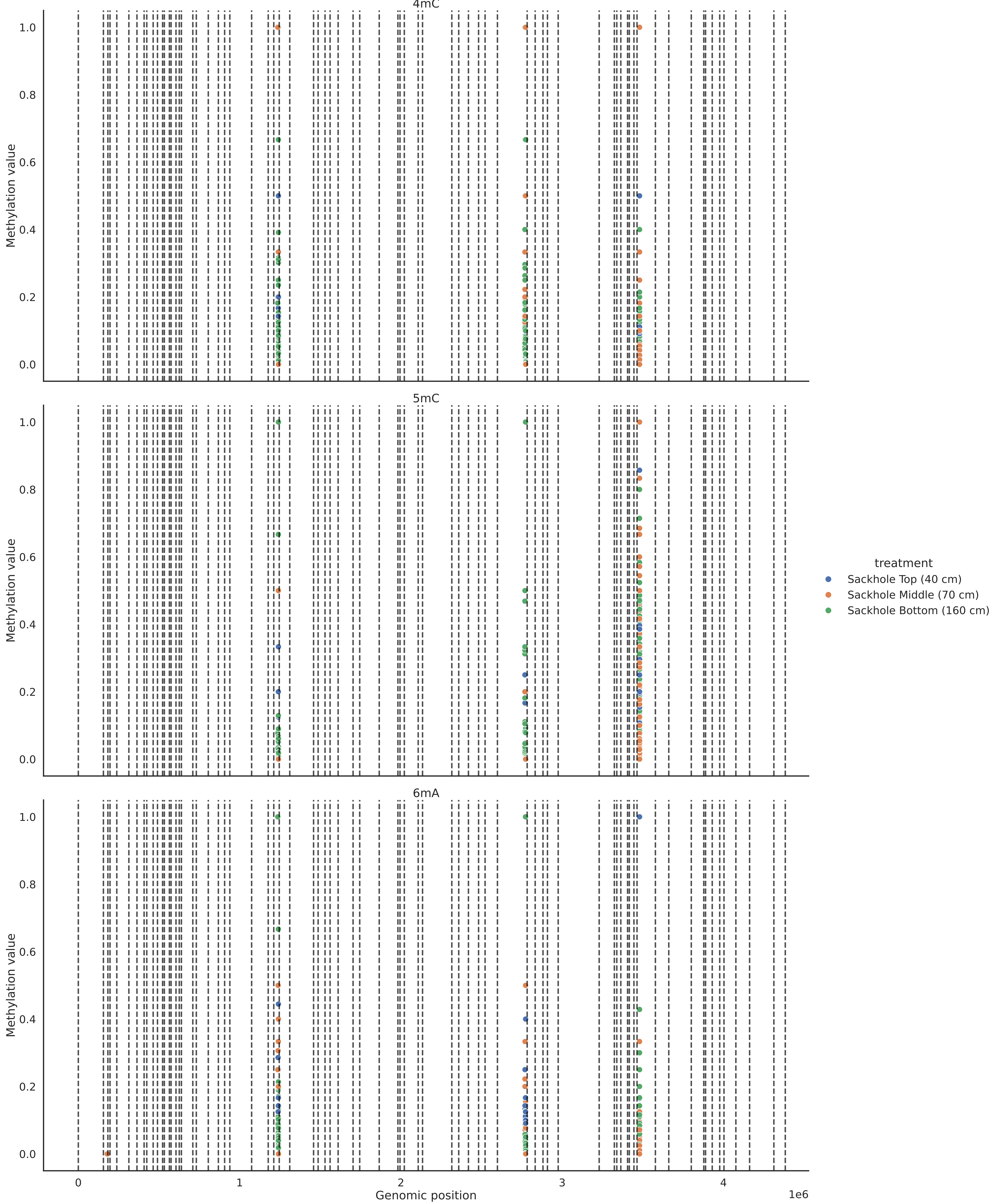
Methylation value across genome of common positions in Rubritalea sp. coverage 2
