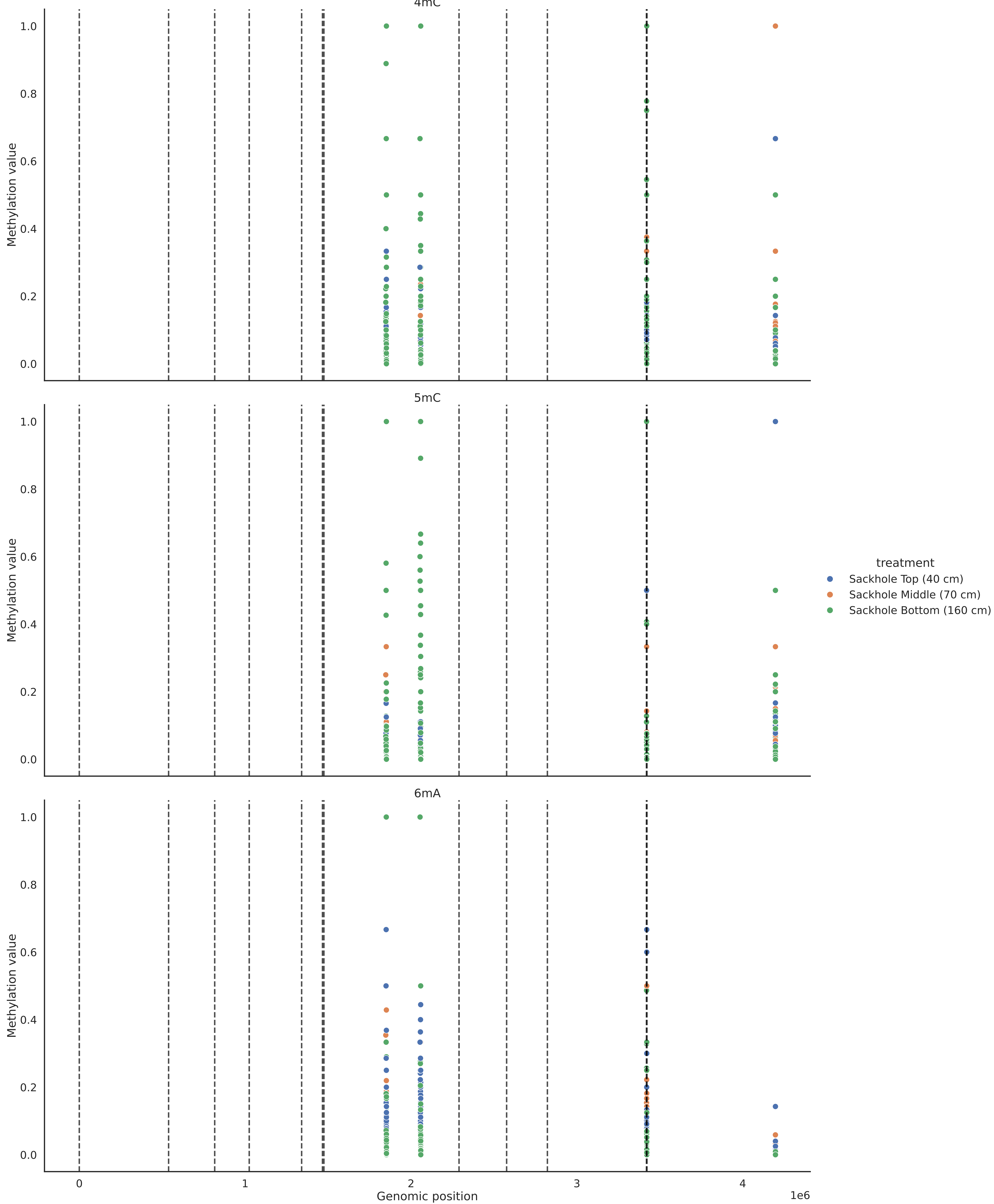
Methylation value across genome of common positions in Halopseudomonas sp. coverage 2
