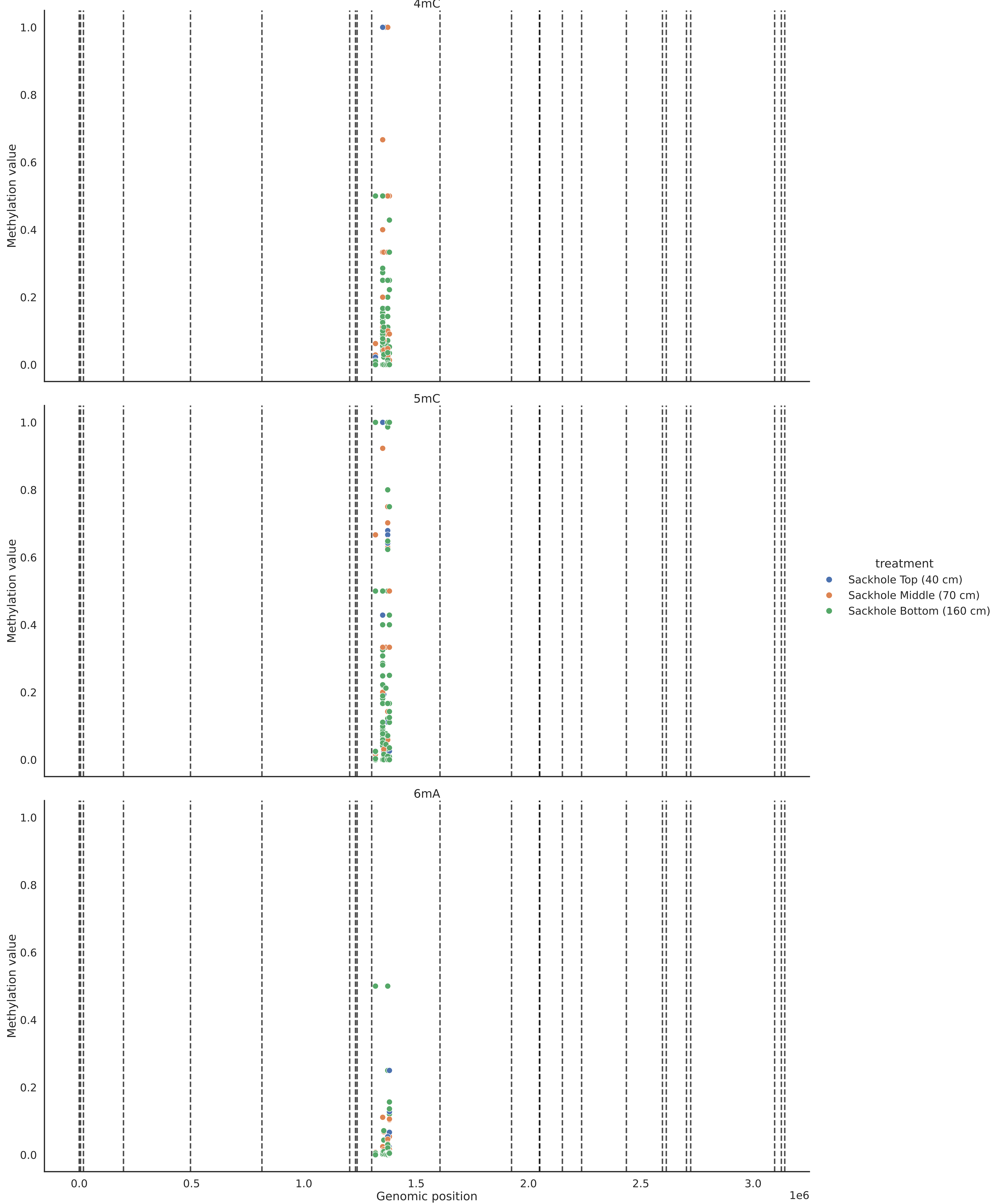
Methylation value across genome of common positions in Polaribacter sp. coverage 7
