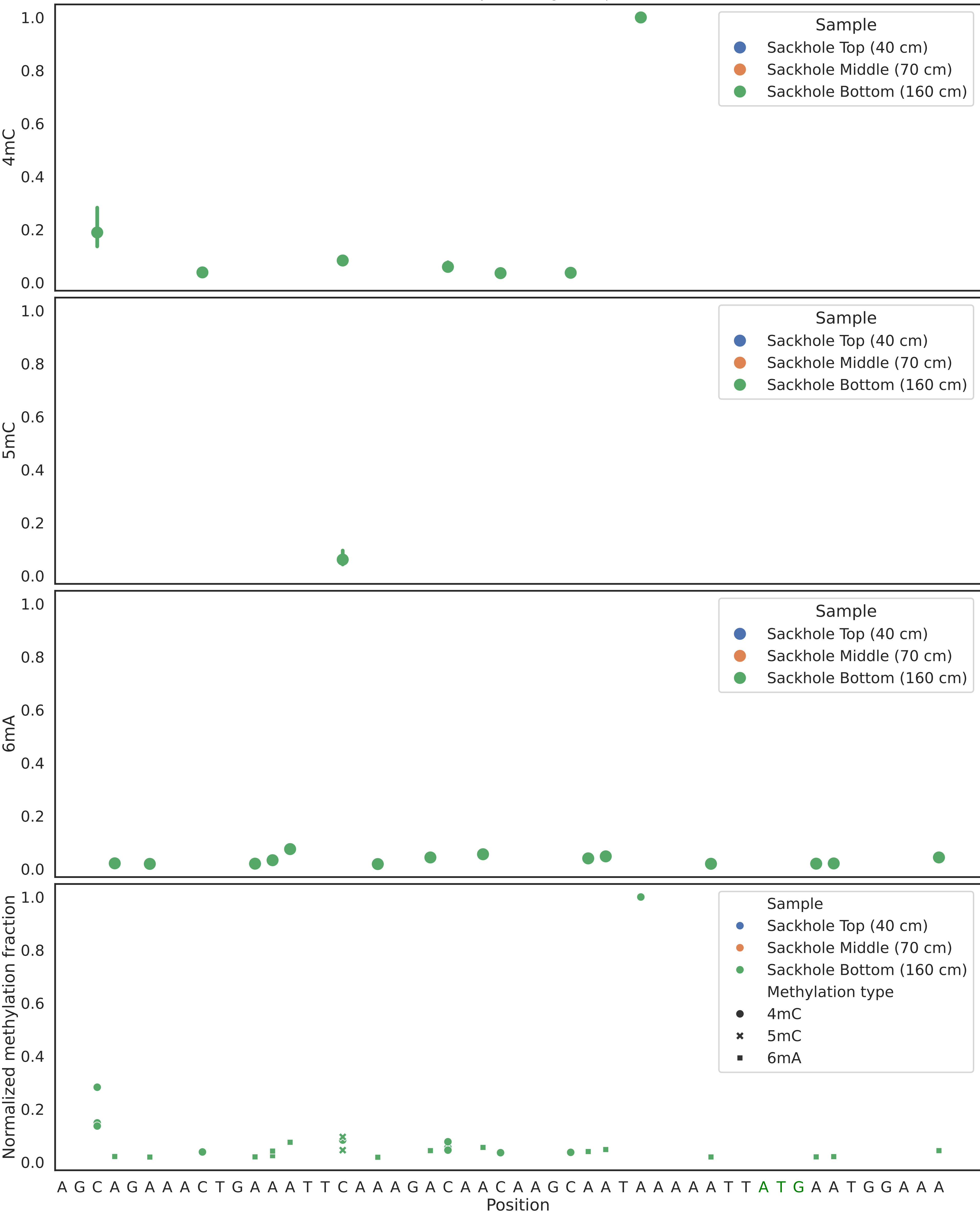
Gene 2435785 methylation - Pelagibacter sp.
