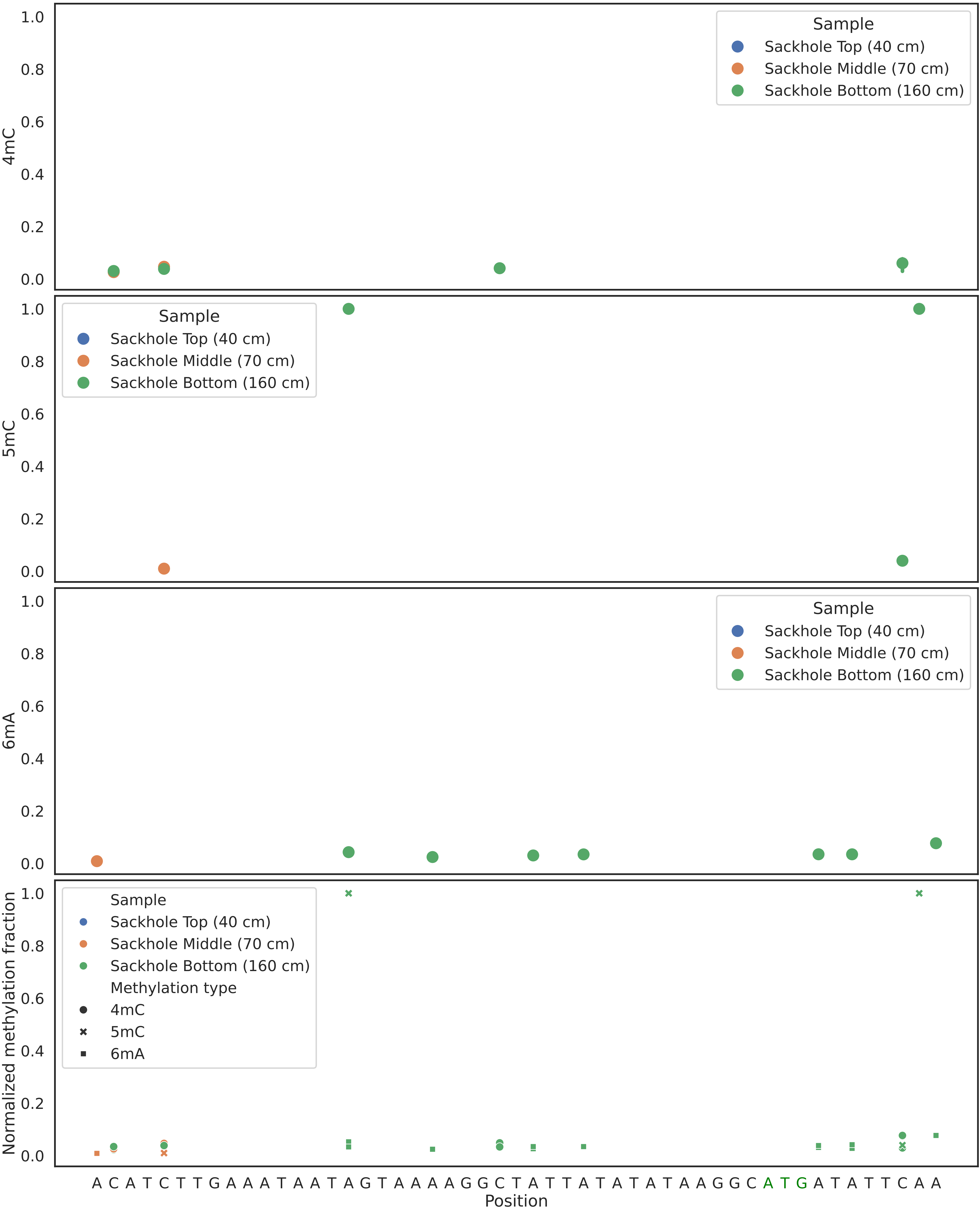
Gene 2435867 methylation - Pelagibacter sp.
