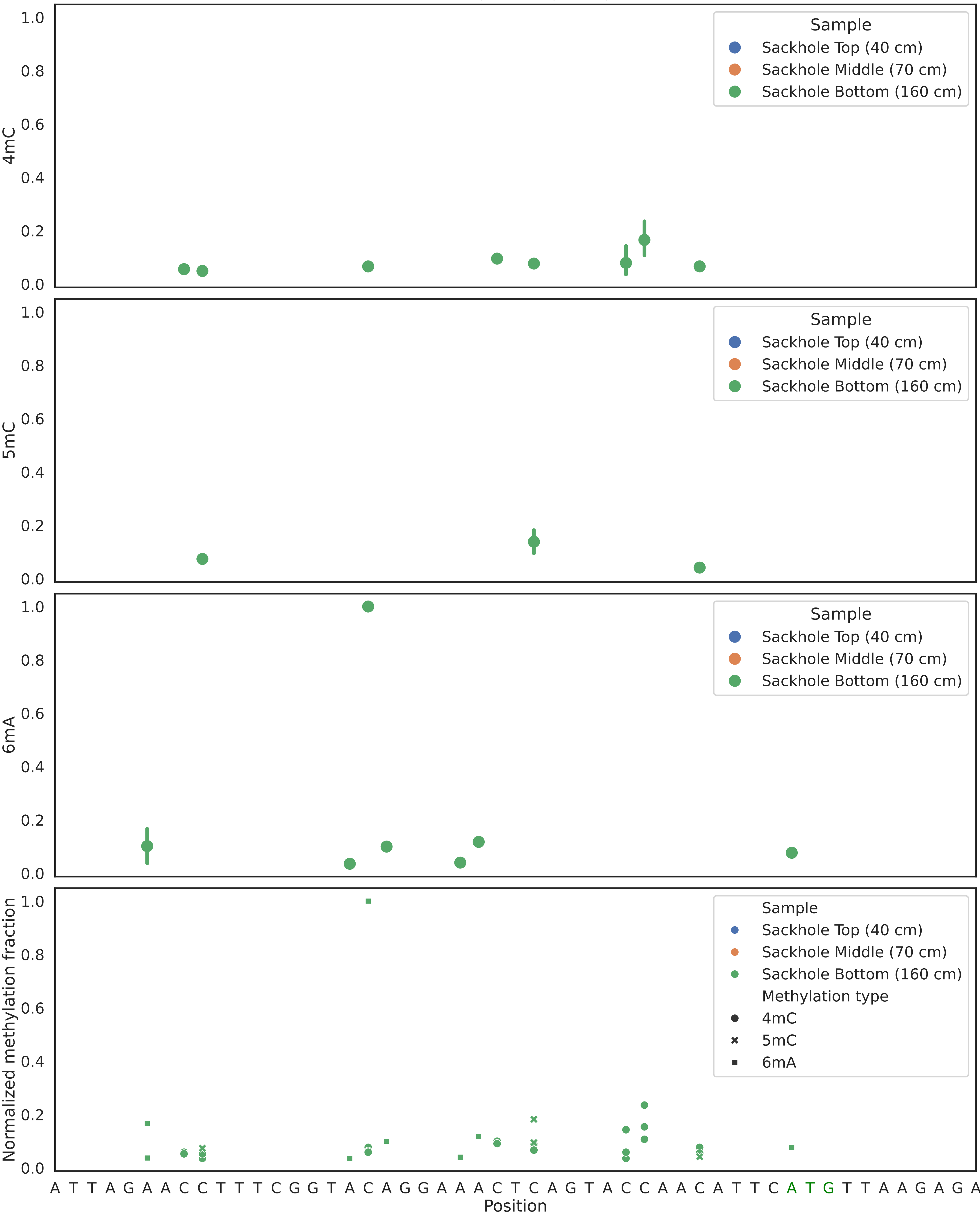
Gene 2442383 methylation - Pelagibacter sp.
