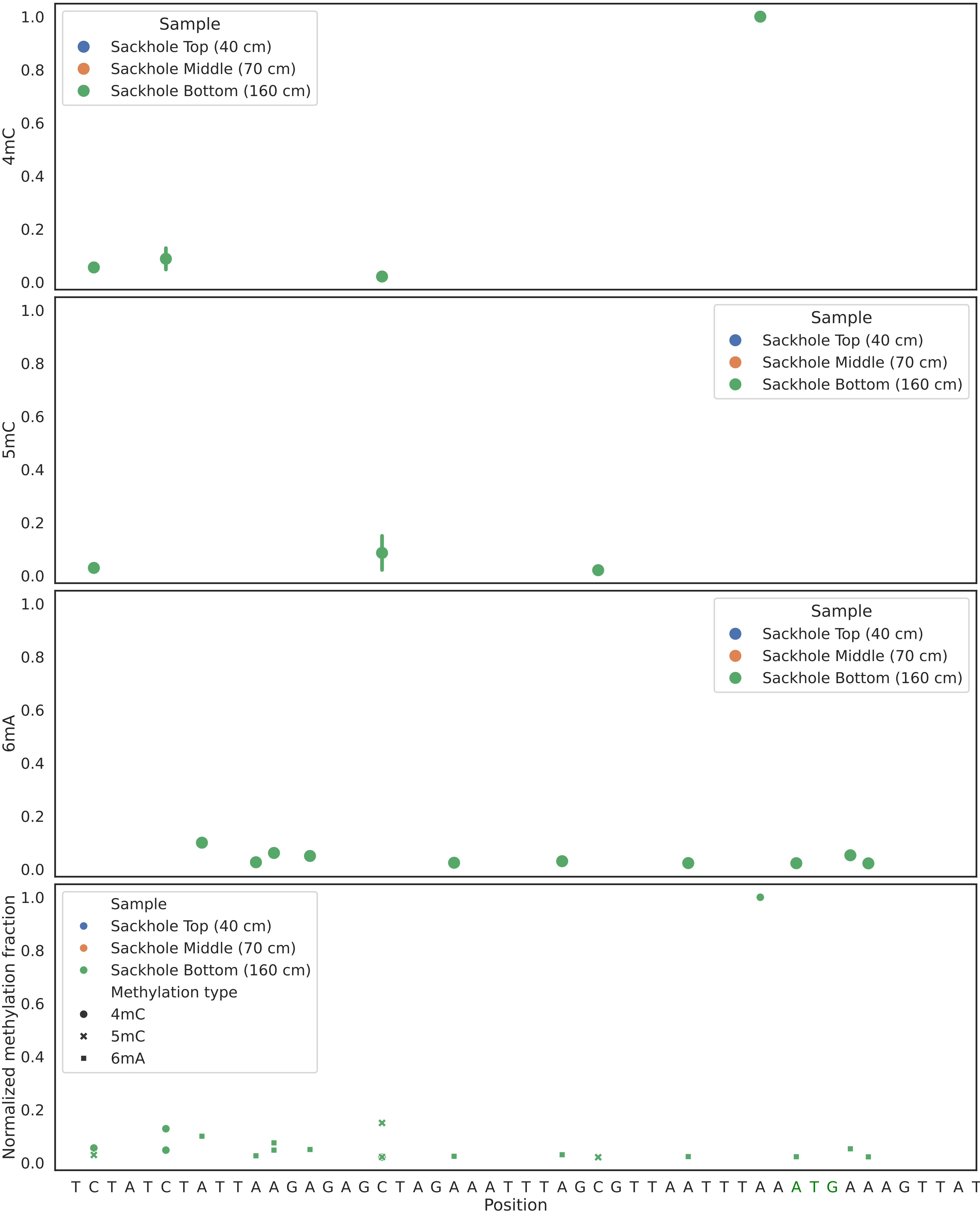
Gene 2451227 methylation - Pelagibacter sp.
