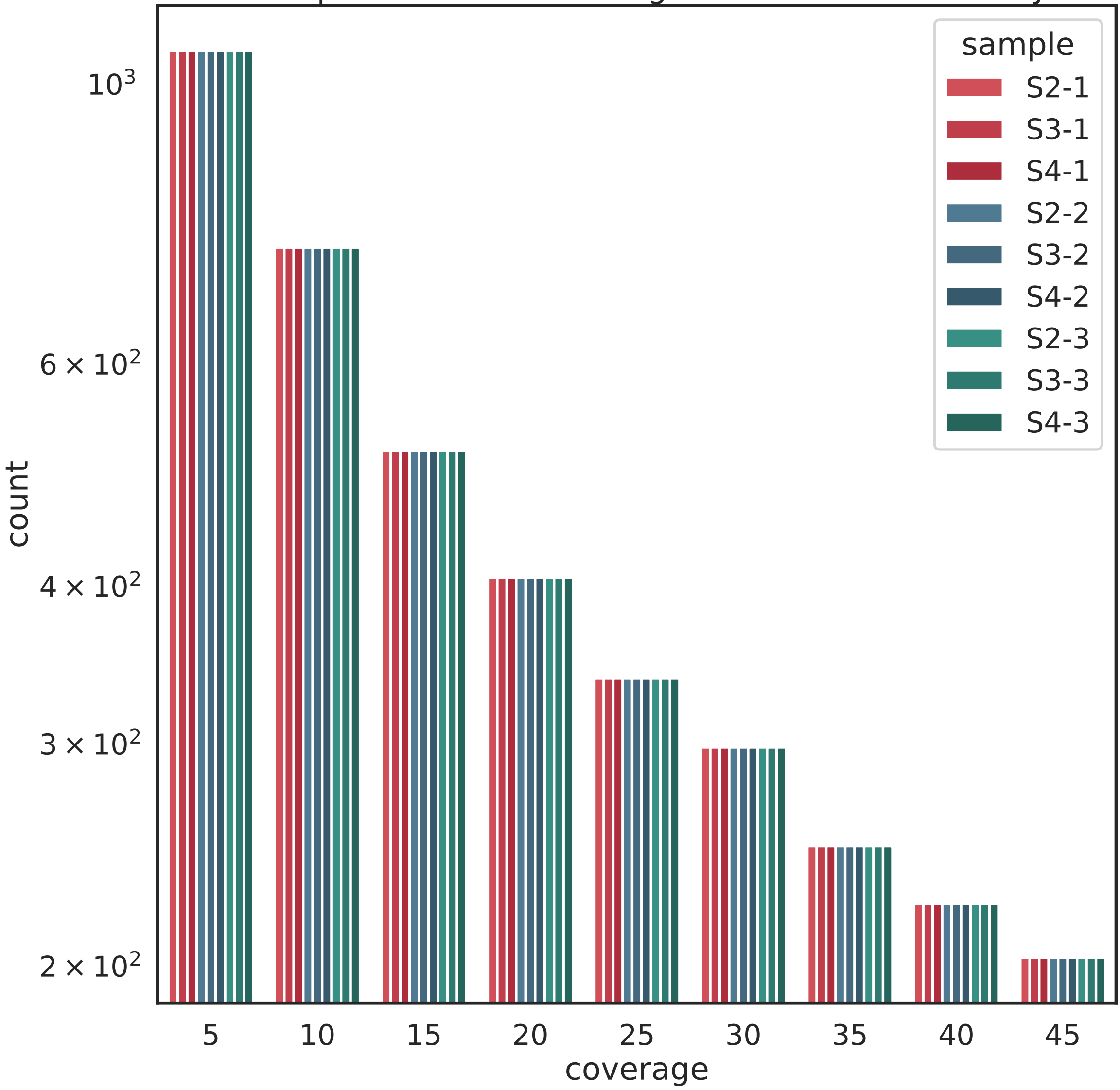
Number of common positions with coverage above threshold in Psychro
