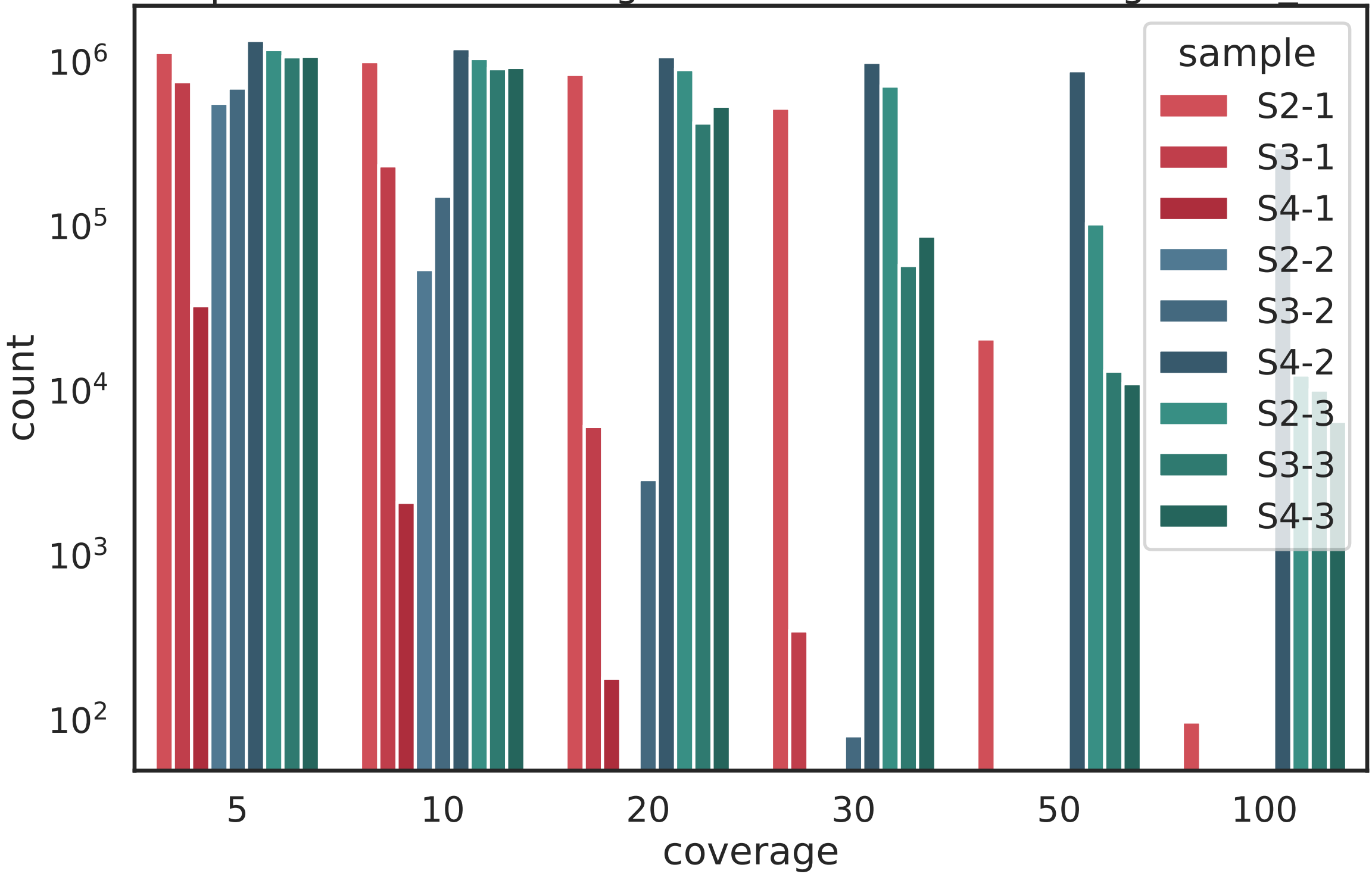
Number of positions with coverage above threshold in Pelagibacter nov
