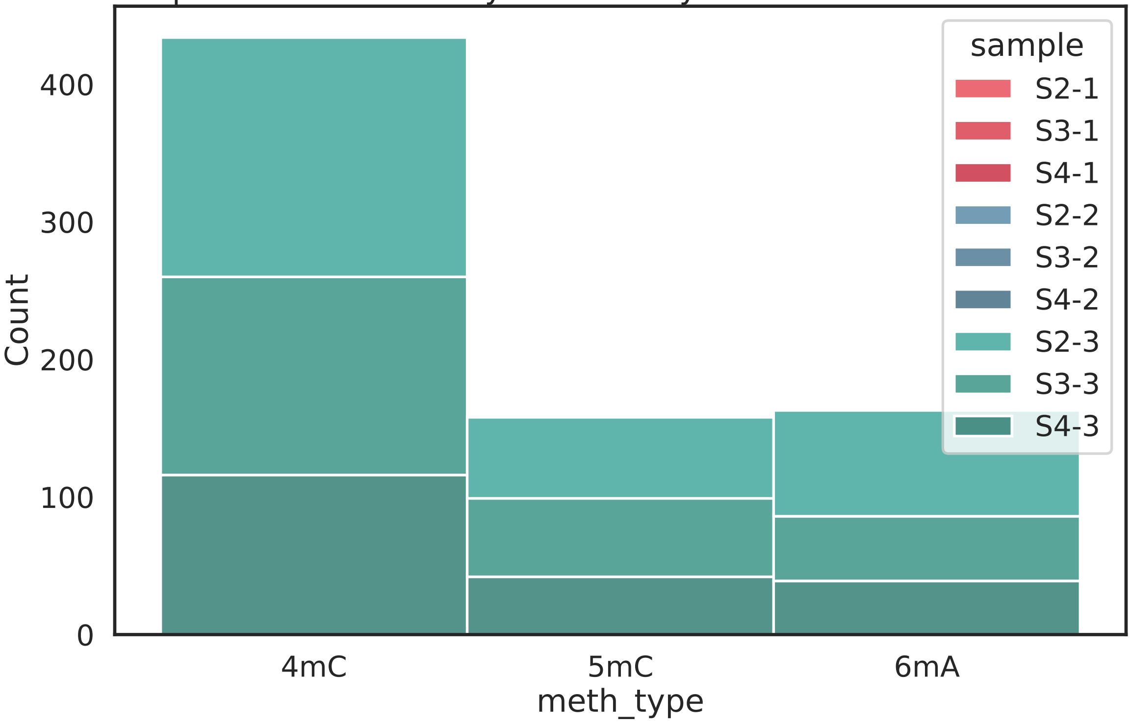
Number of positions 95% methylated in only 1 treatment in Brevundimor
