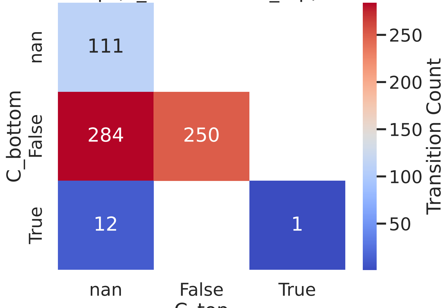
on Heatmap (C_bottom vs. C_top) in Rubritalea s
