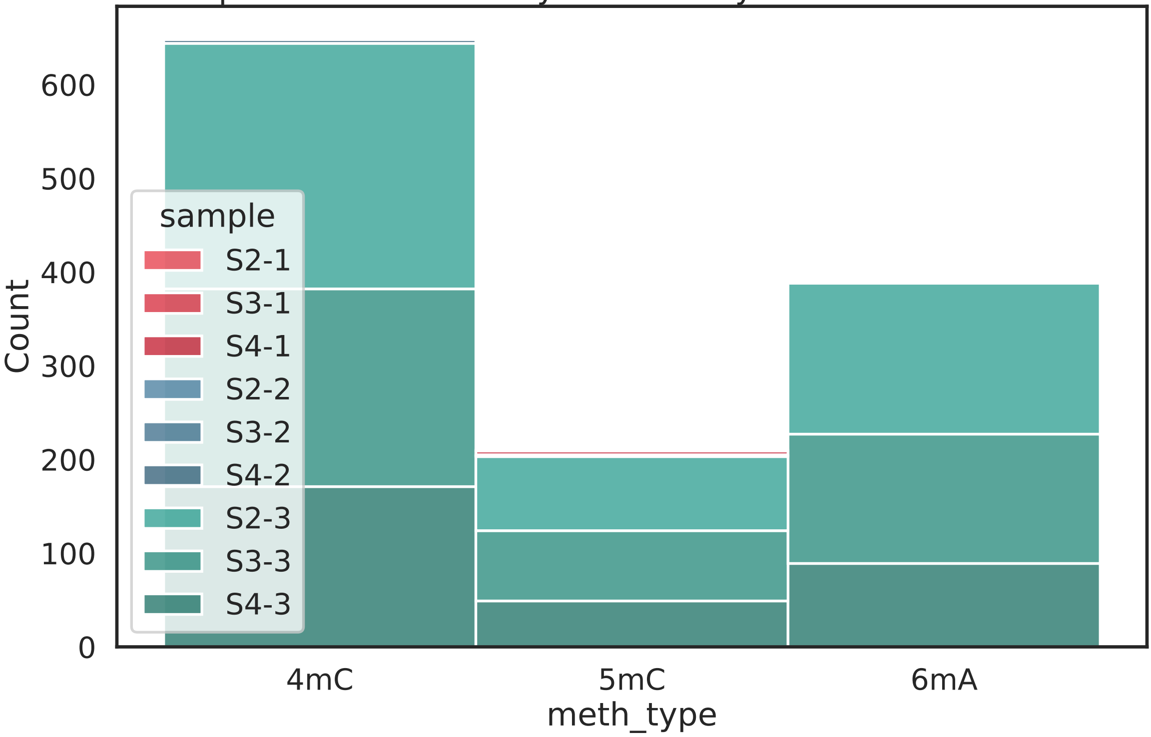
Number of positions 95% methylated in only 1 treatment in Rubritale
