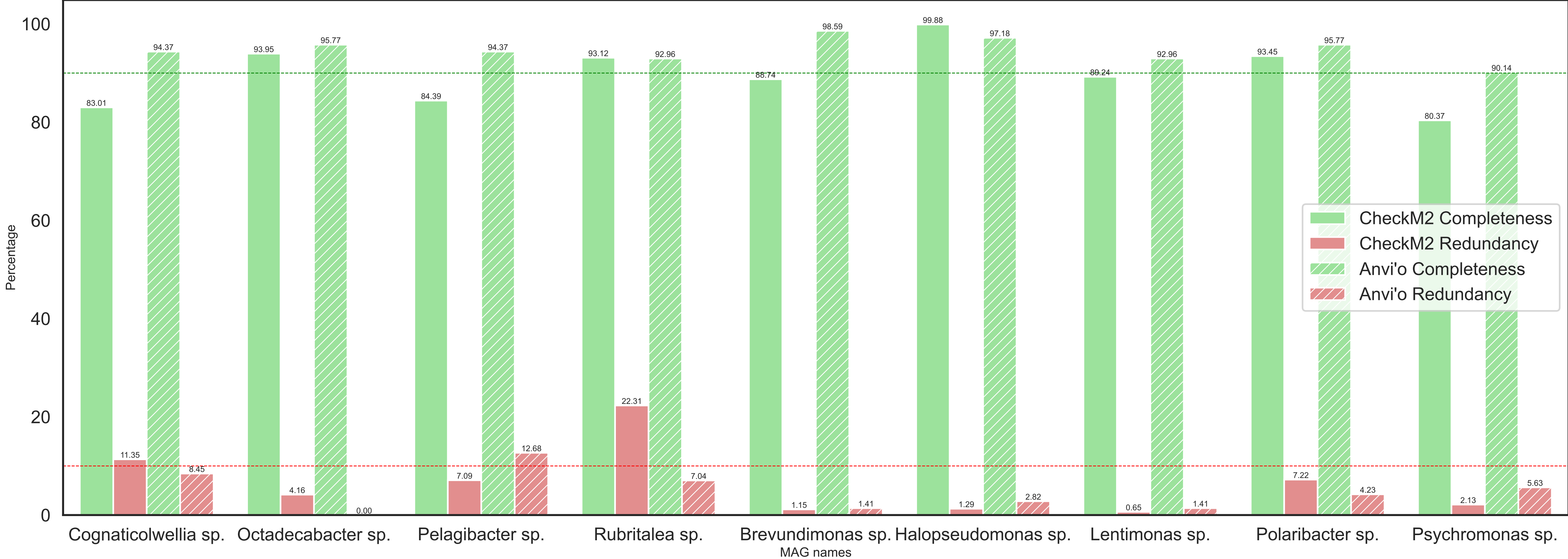
MAG quality assessment
