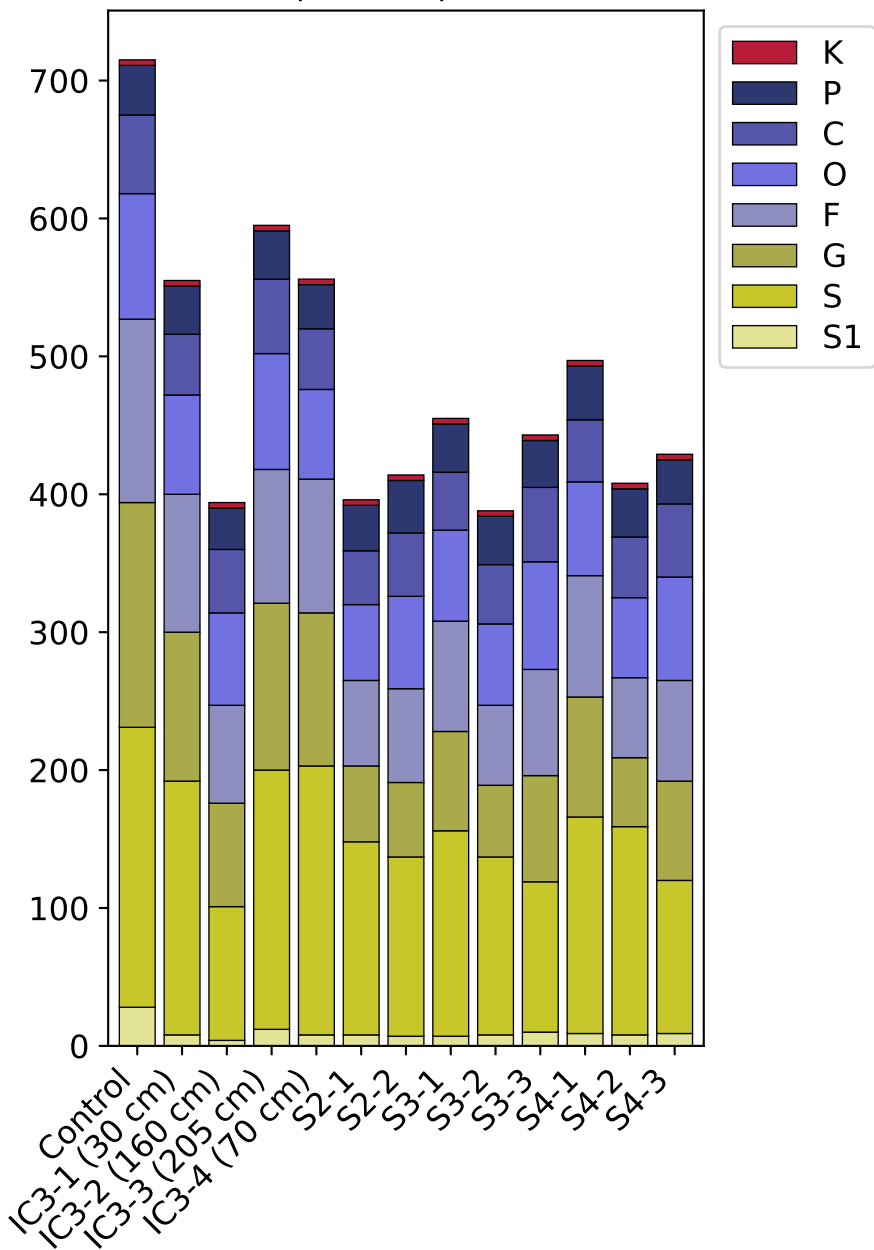
Unique-Taxa-per-Rank
