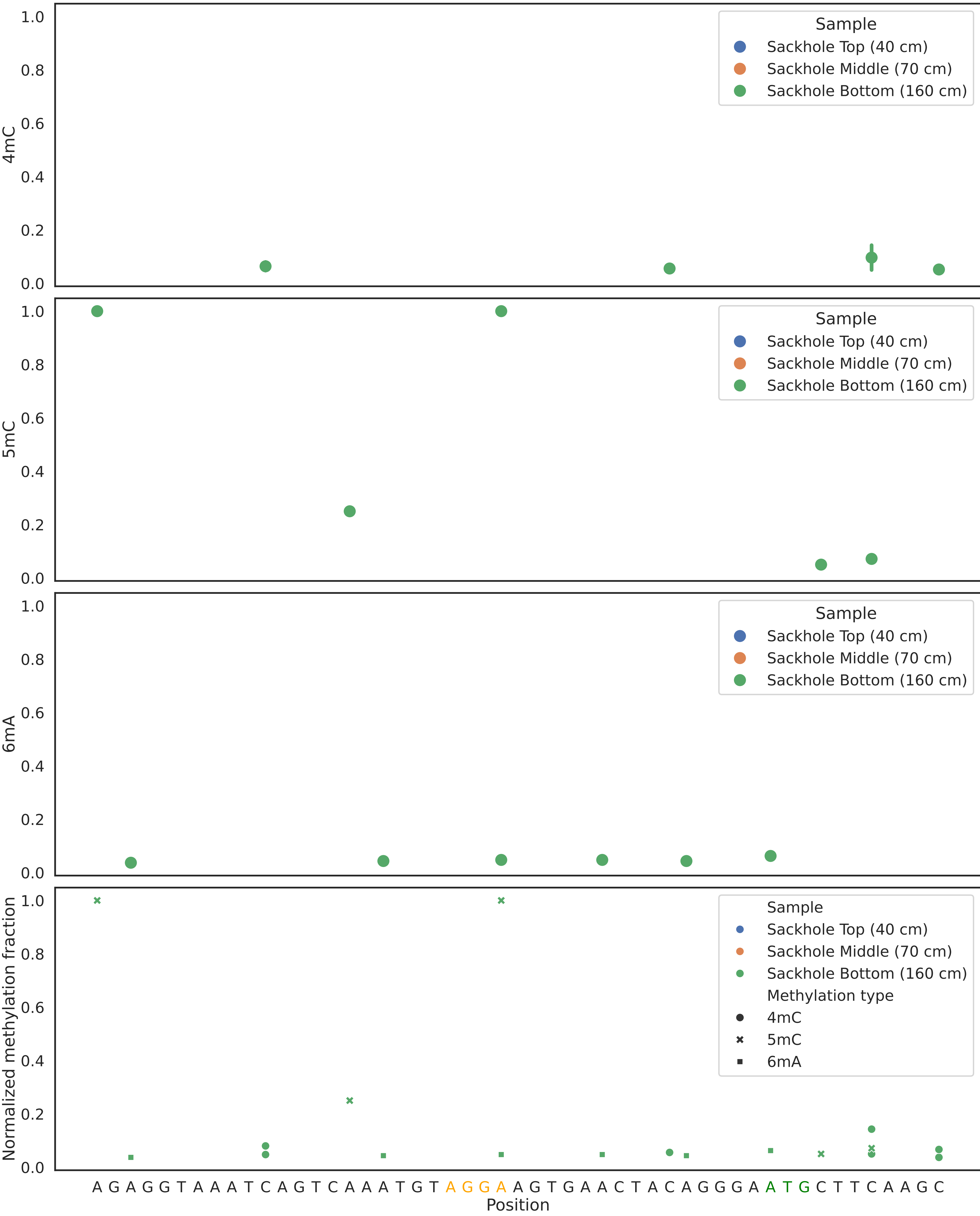
Gene 2538698 methylation - Pelagibacter sp.
