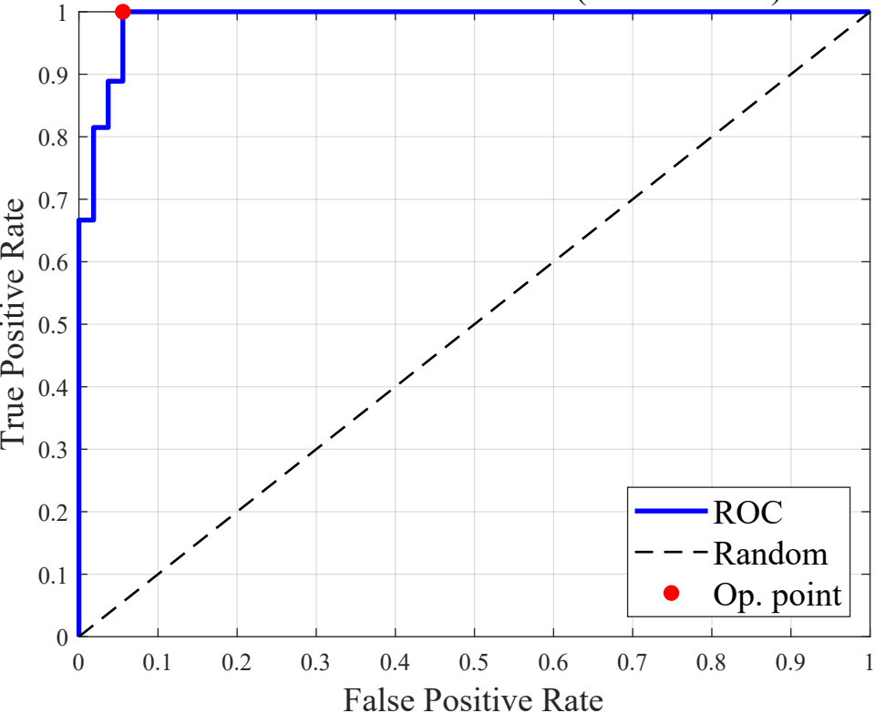
ROC for Unknown Detection (AUC = 0.988)
