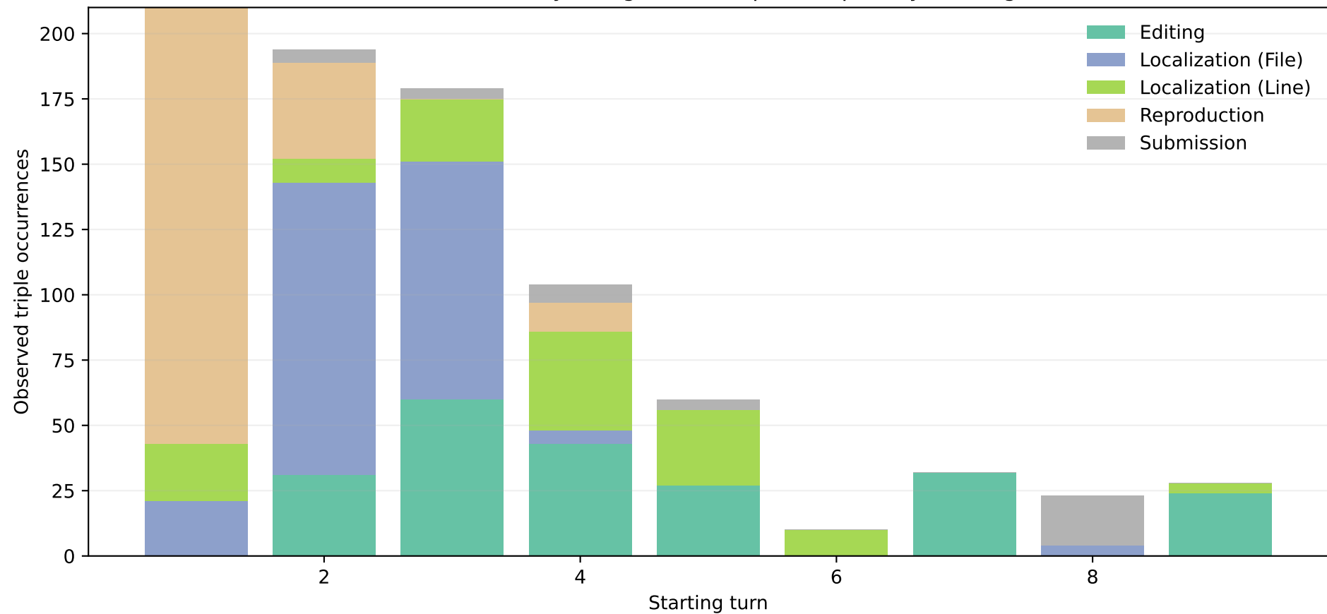
Published manually categorized frequent triples by starting turn
