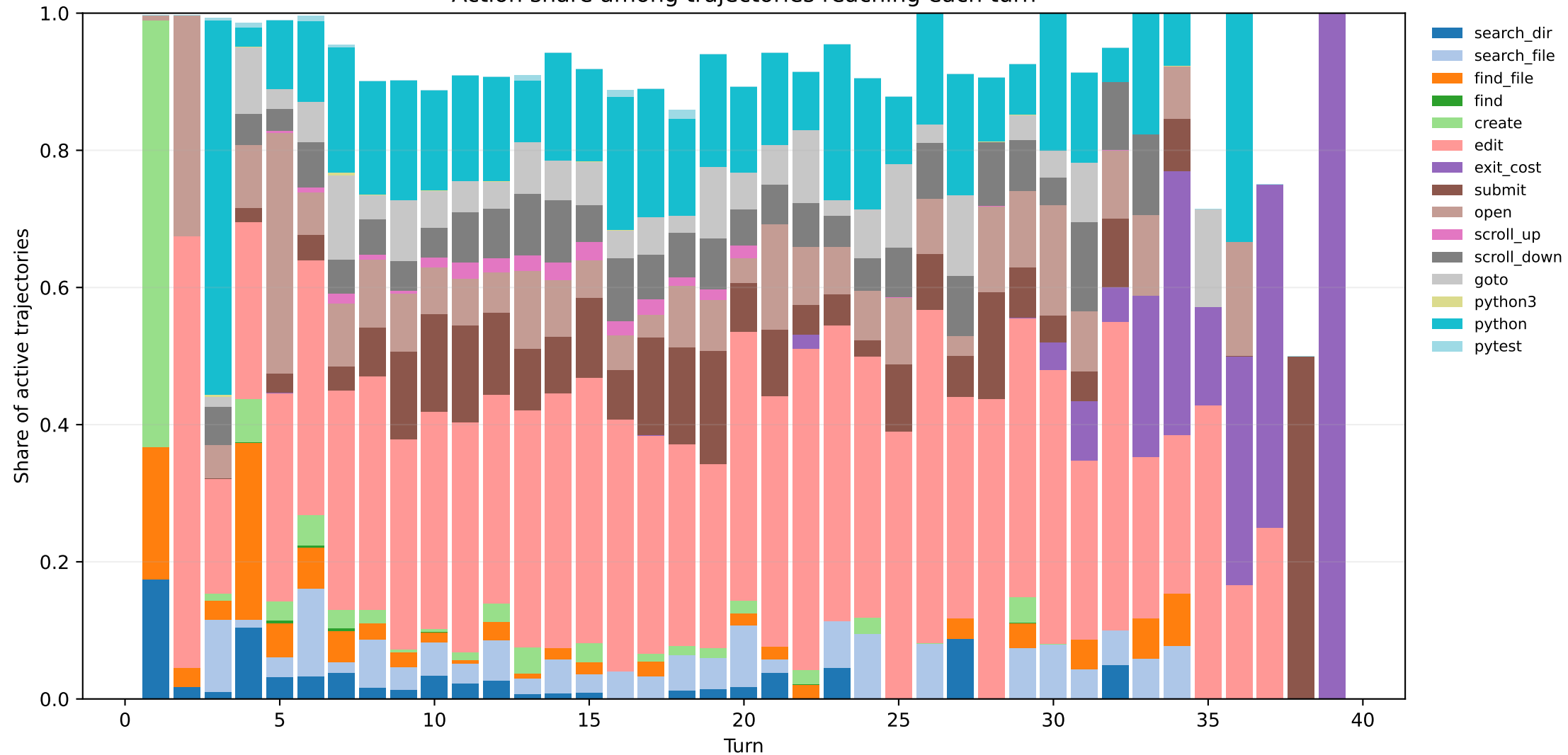
Action share among trajectories reaching each turn
