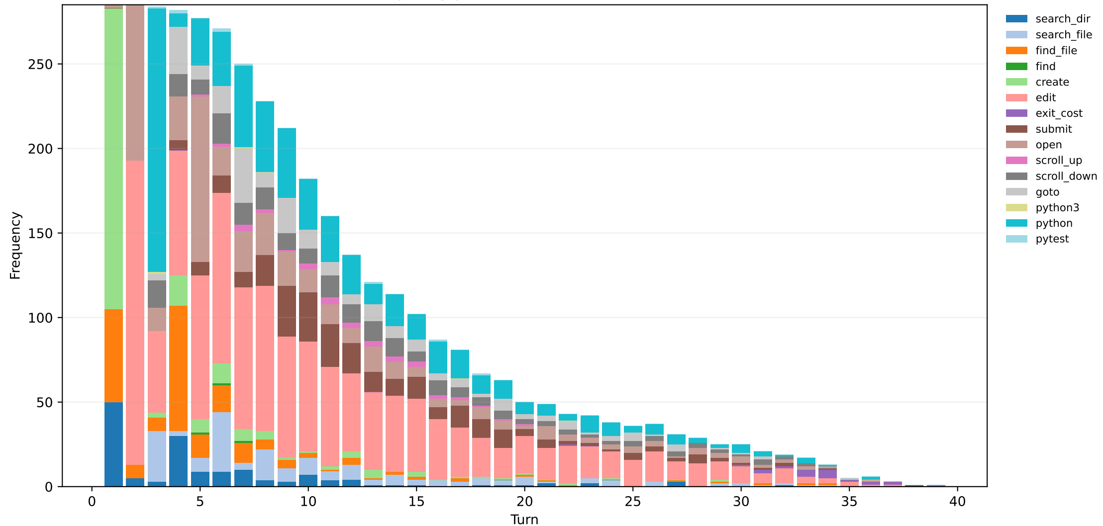
Action frequency per turn / resolved GPT-4 Turbo Full
