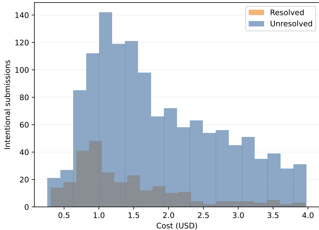
Intentional submissions before budget exhaustion / GPT-4 Turbo Full
