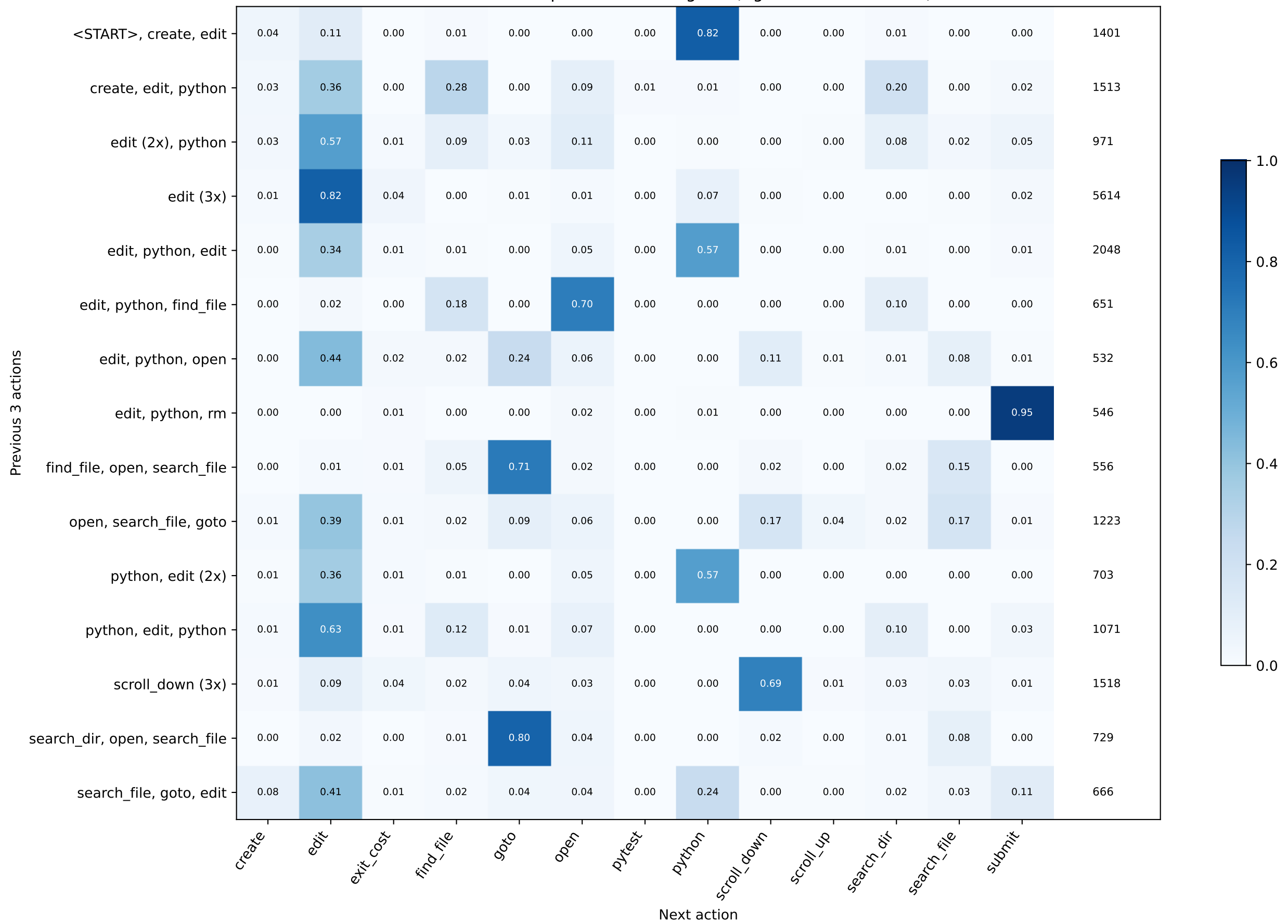
Transition probabilities / 3-gram (right counts corrected)
