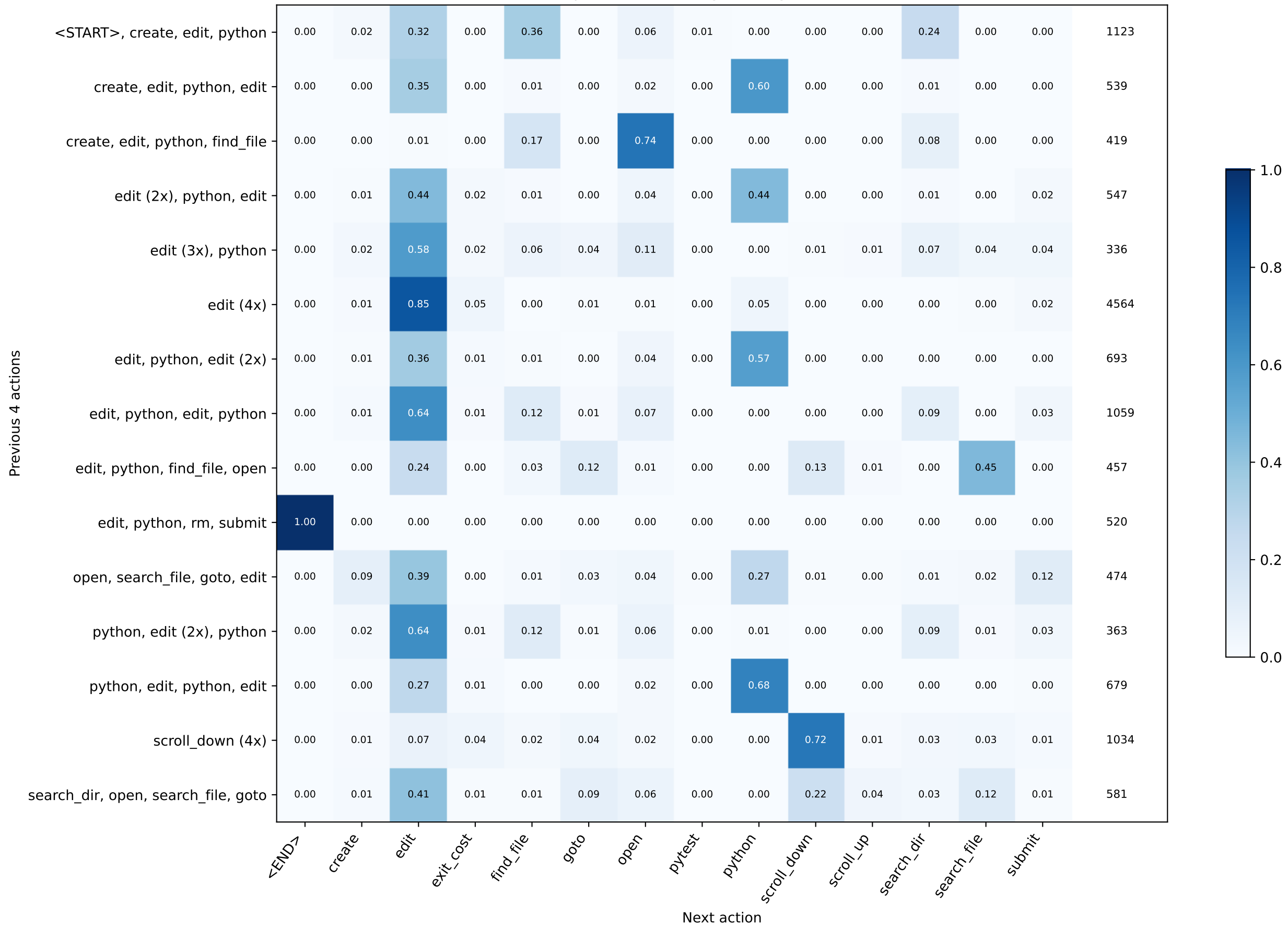
Transition probabilities / 4-gram (right counts corrected)
