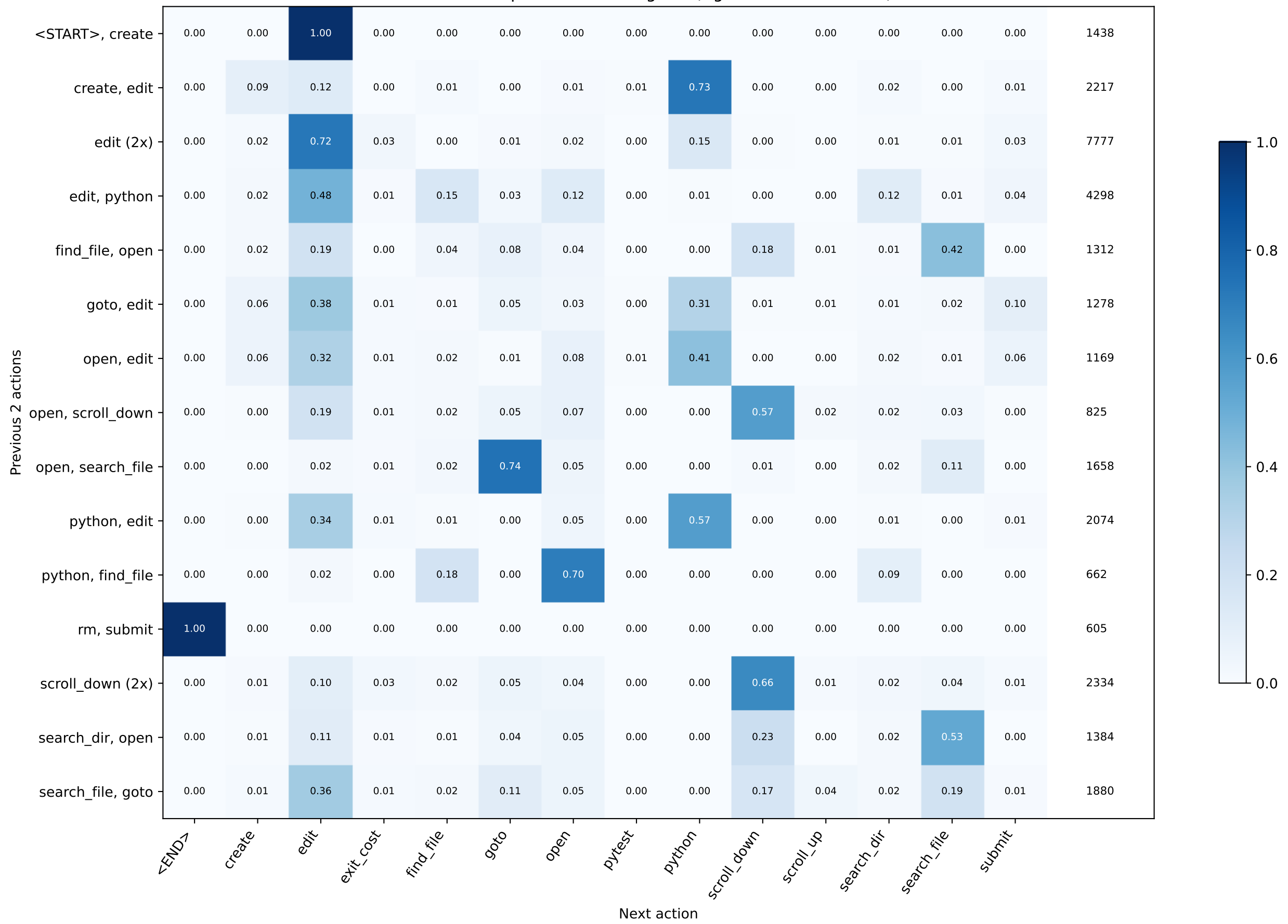
Transition probabilities / 2-gram (right counts corrected)
