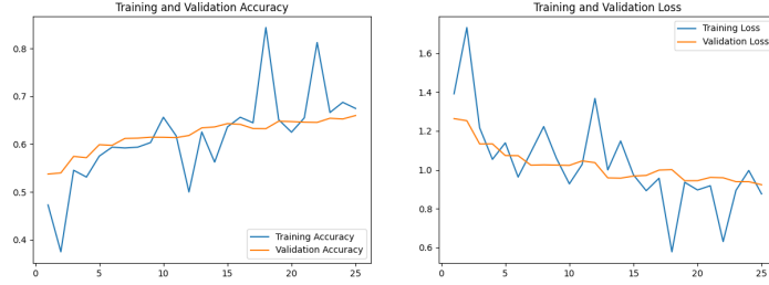
Figure 10: Model A — Training and validation accuracy and loss (7 classes, 25 epochs).
