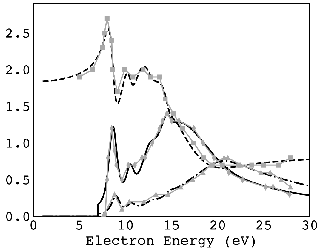
Hexagonal Ice
