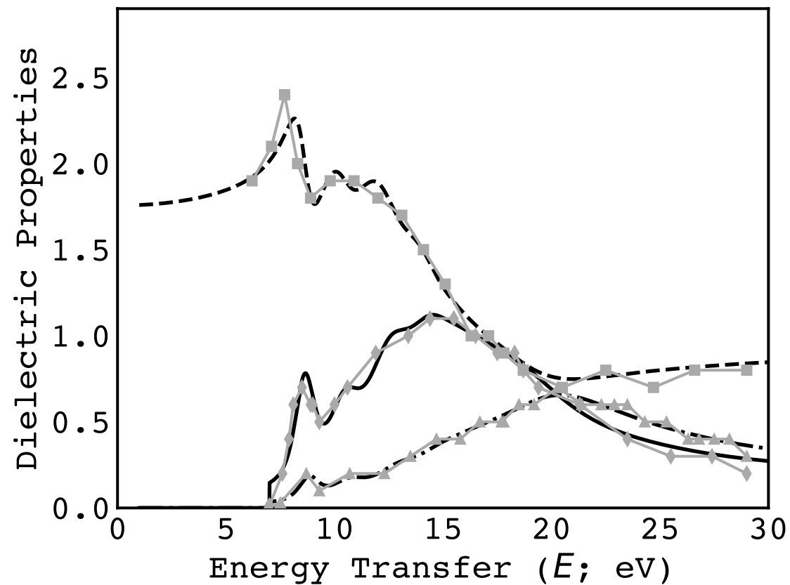
Amorphous Ice
