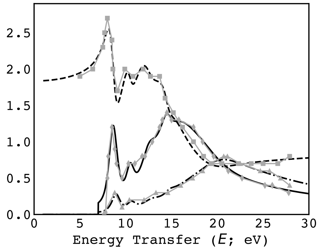
Hexagonal Ice
