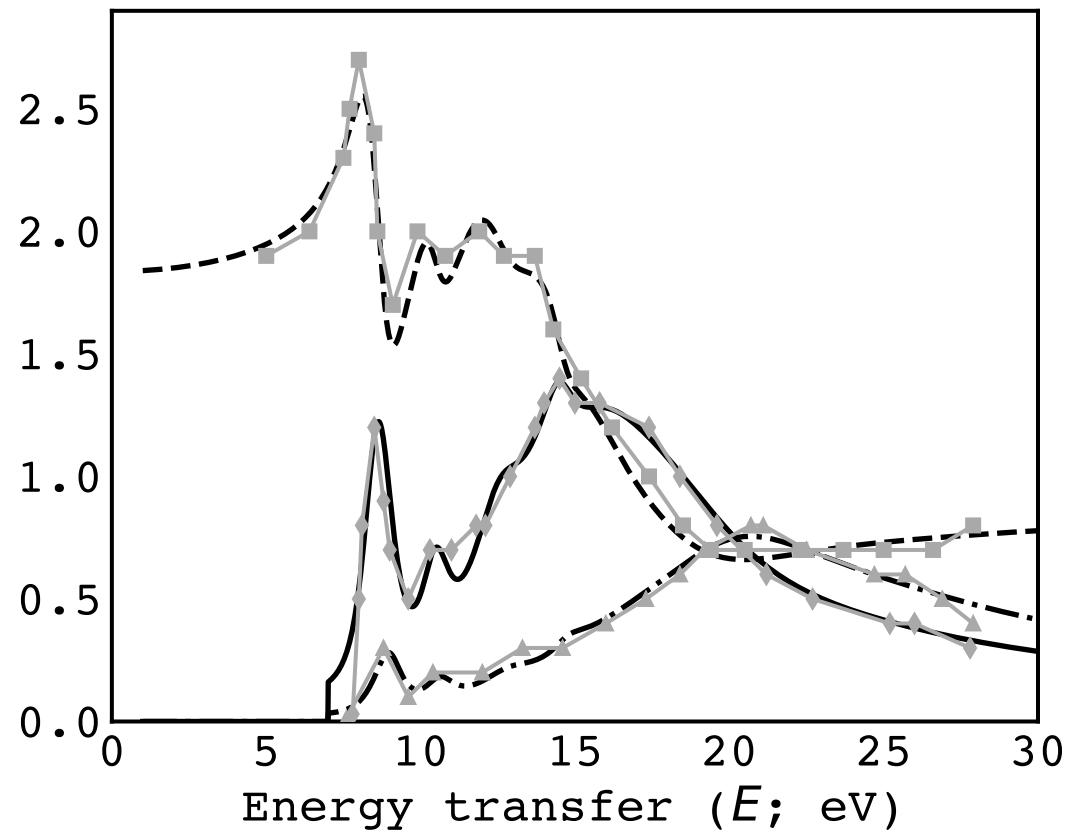
Hexagonal ice
