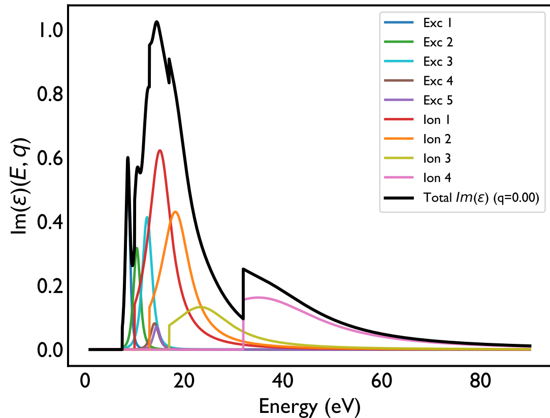
Channel-resolved \text{Im}(\epsilon) at q = 0.00 ; amorphous ice
