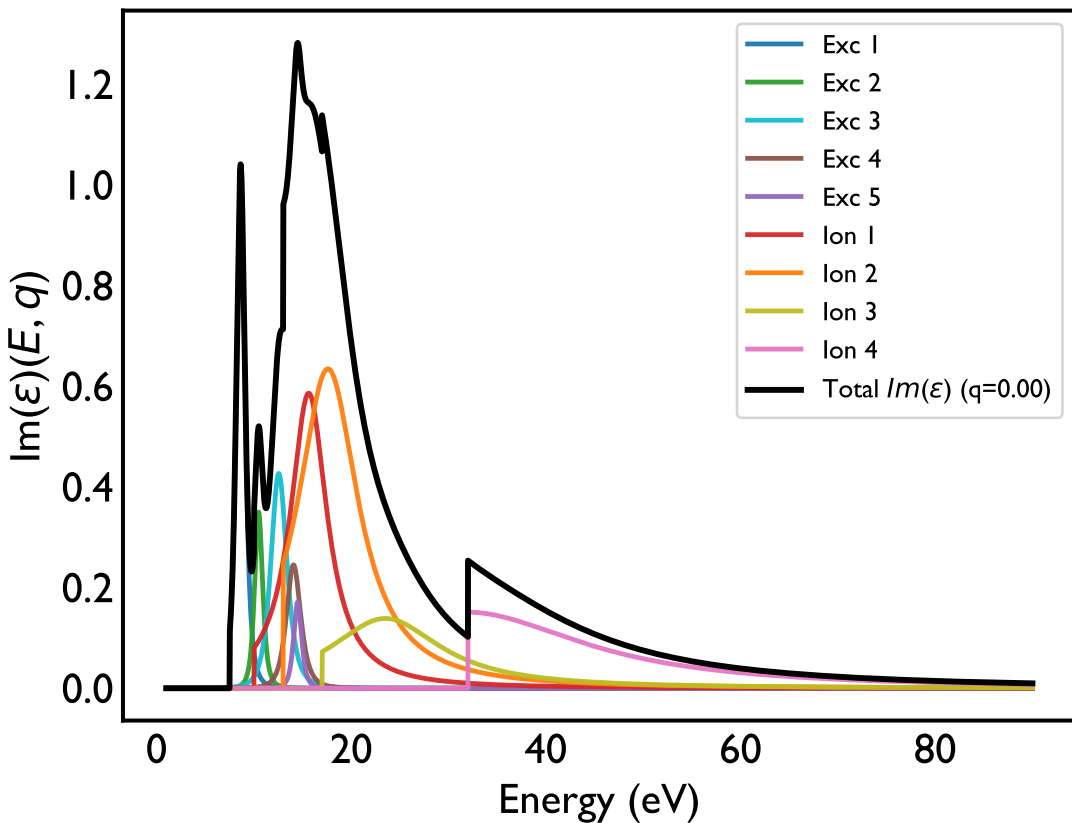
Channel-resolved \text{Im}(\epsilon) at q = 0.00 ; hexagonal ice
