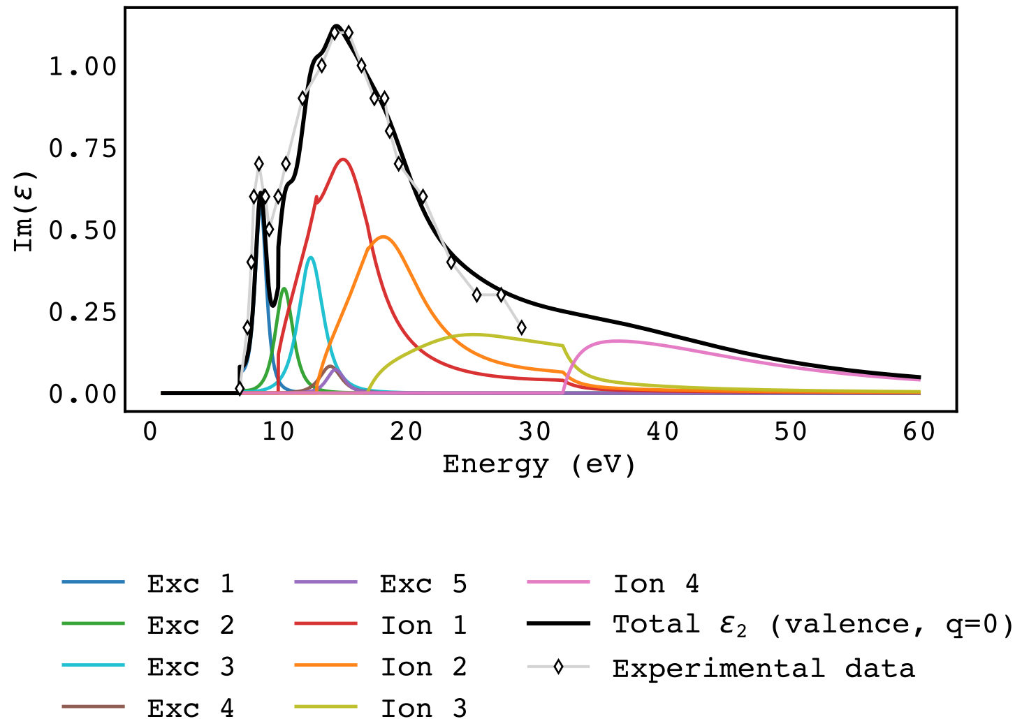
Channel-resolved \text{Im}(\epsilon) at q = 0.0 ; amorphous ice
