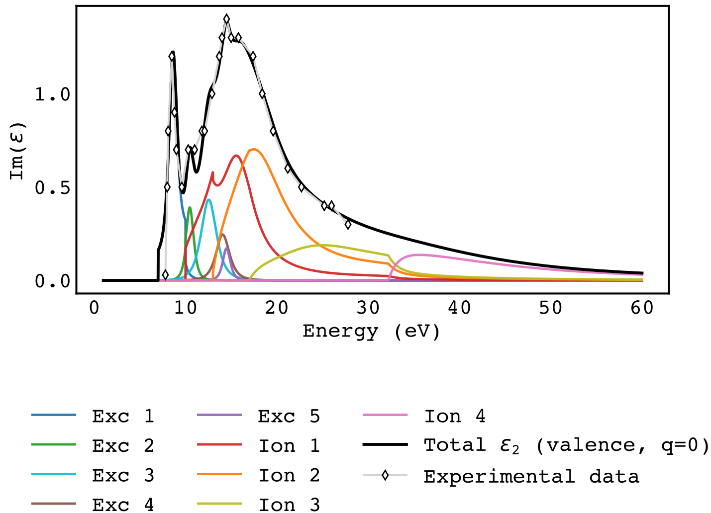
Channel-resolved \text{Im}(\varepsilon) at q = 0.0 ; hexagonal ice
