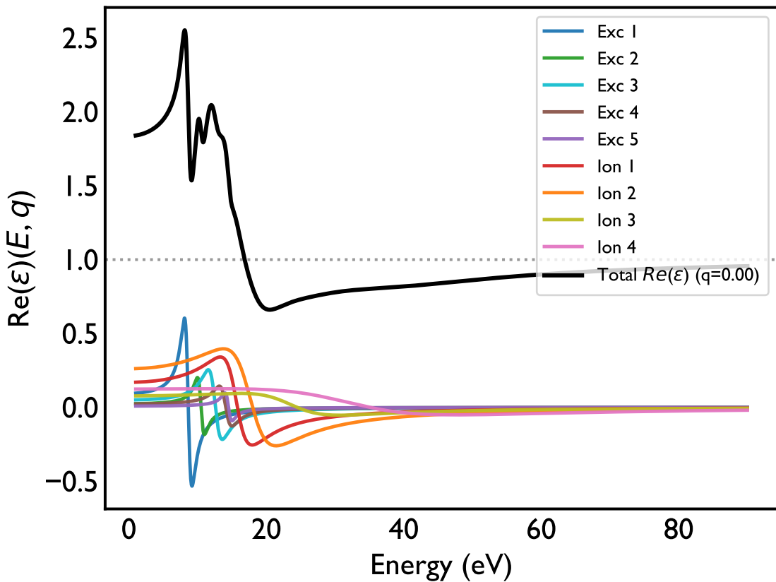
Channel-resolved \text{Re}(\epsilon) at q = 0.00 ; hexagonal ice
