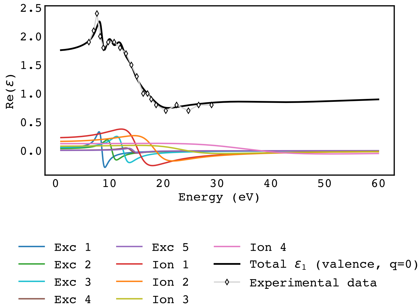
Channel-resolved \text{Re}(\epsilon) at q = 0.0 ; amorphous ice
