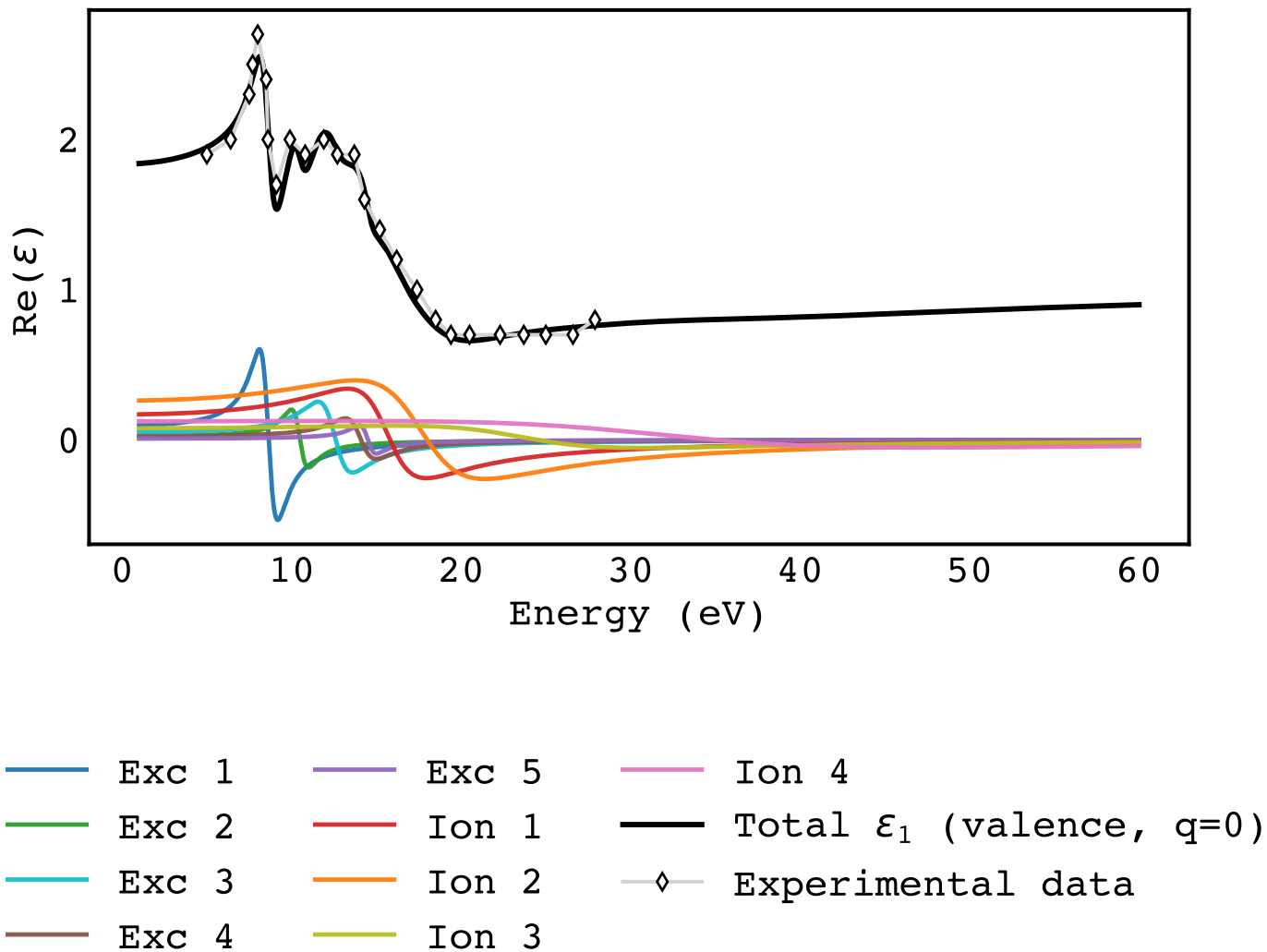
Channel-resolved \text{Re}(\epsilon) at q = 0.0 ; hexagonal ice
