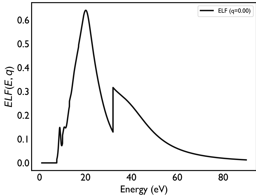
ELF at q = 0.00 with O K-shell; amorphous ice
