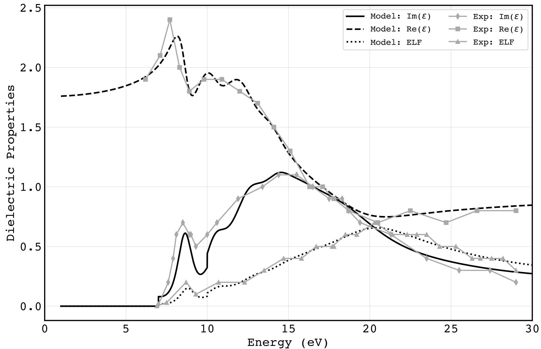
Model vs Experiment: Amorphous Ice (optical limit, q=0 )
