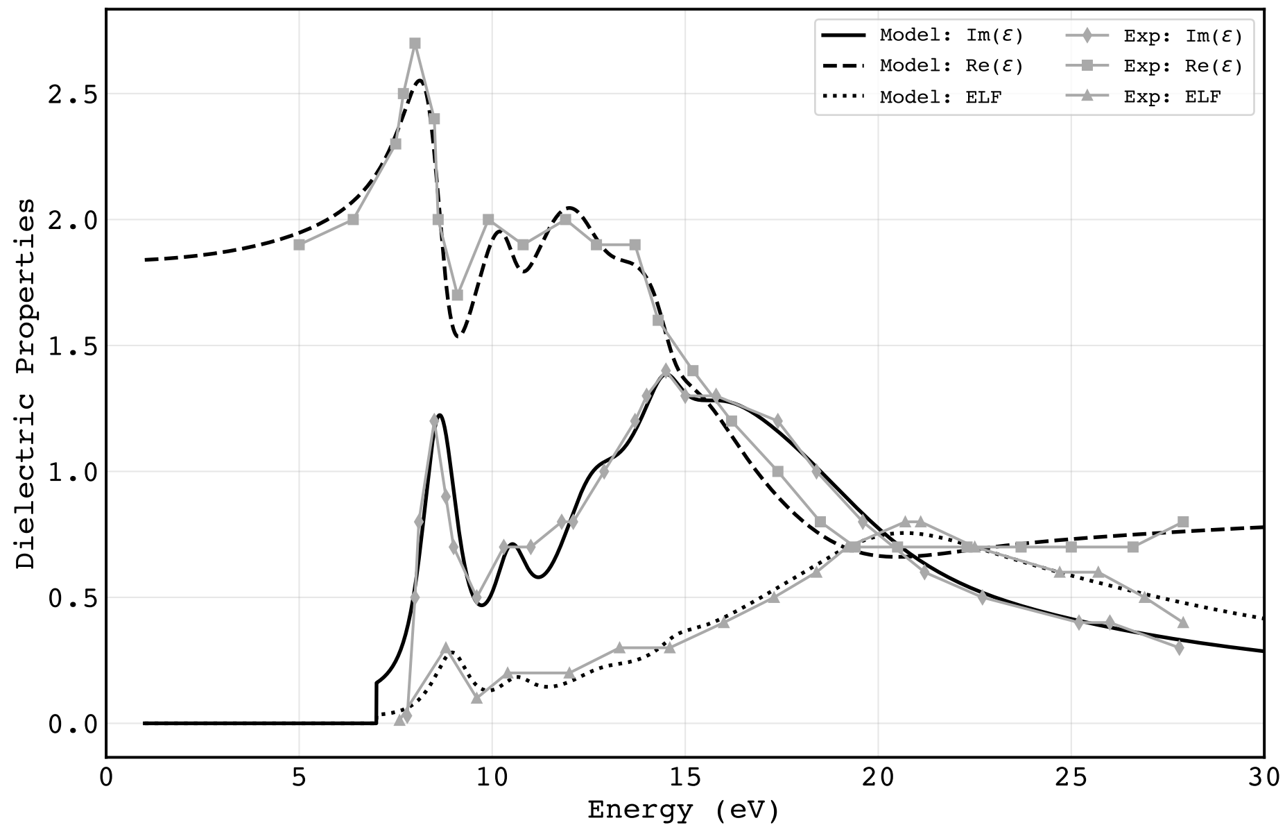
Model vs Experiment: Hexagonal Ice (optical limit, q=0 )
