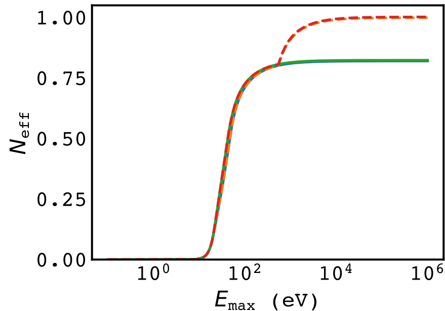
N_{\text{eff}} vs E_{\text{max}}
