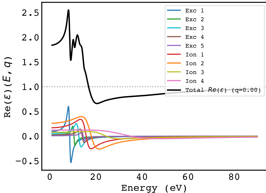
Channel-resolved \text{Re}(\epsilon) at q = 0.00 ; hexagonal ice
