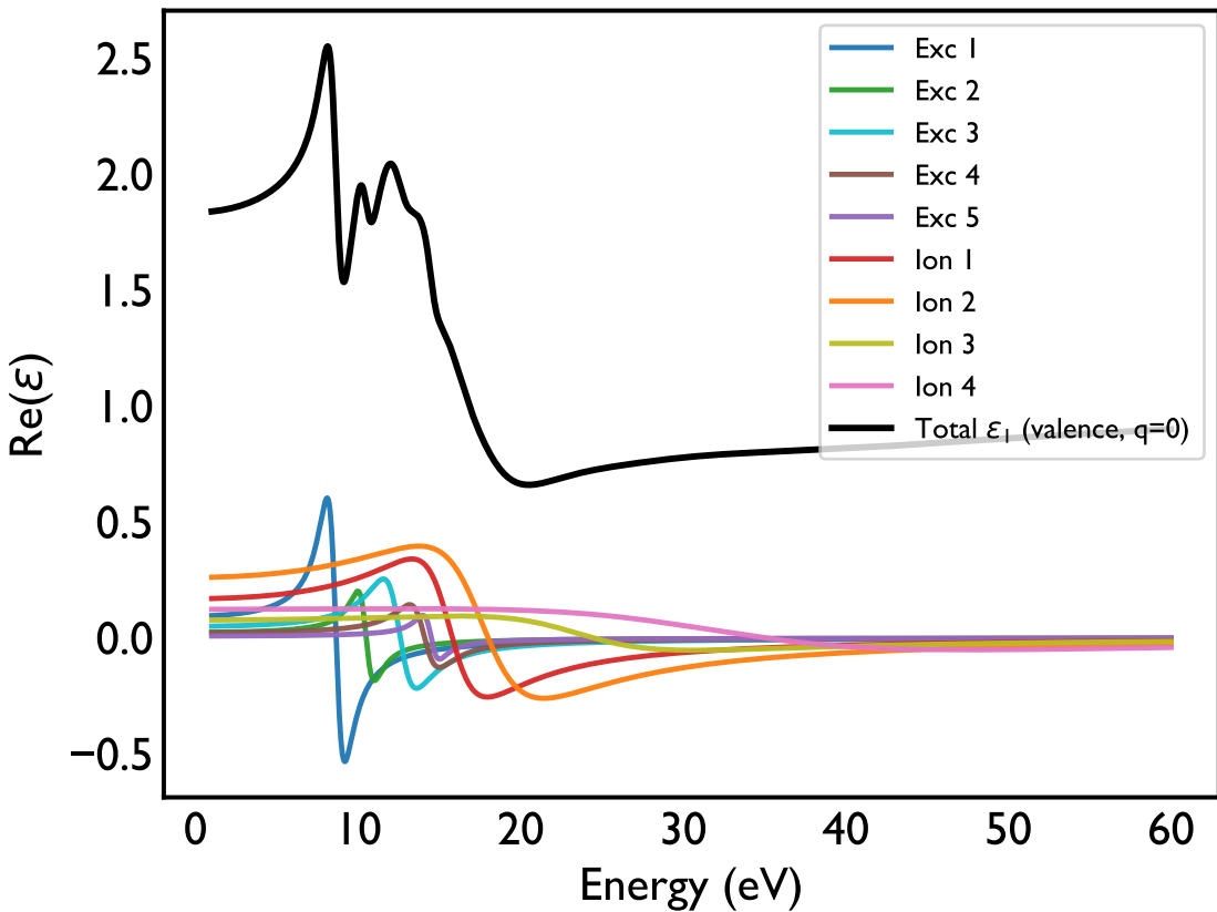
Channel-resolved \text{Re}(\varepsilon) at q = 0.0 ; hexagonal ice
