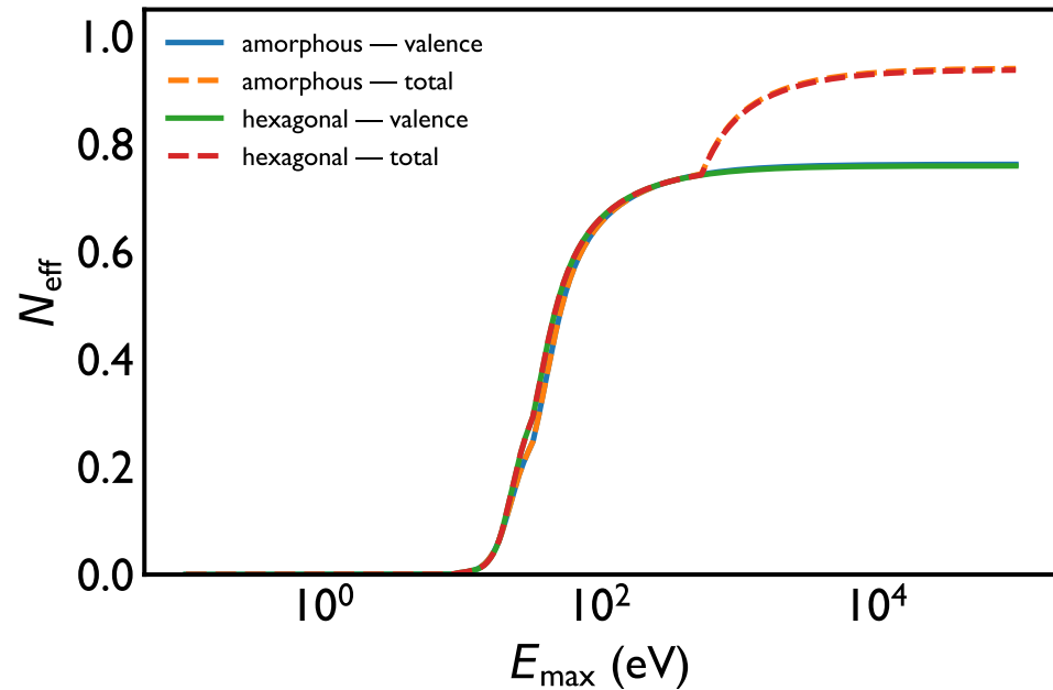
N_{\text{eff}} vs E_{\text{max}}
