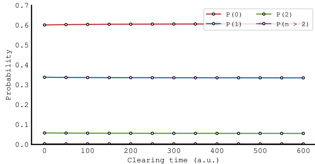
(b) Electrons in projectile sphere
