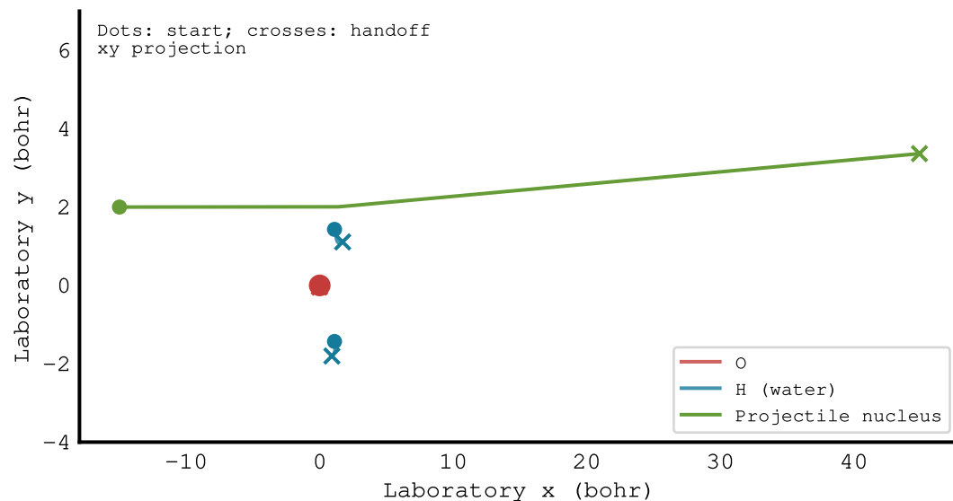
(a) Measured nuclear trajectories
