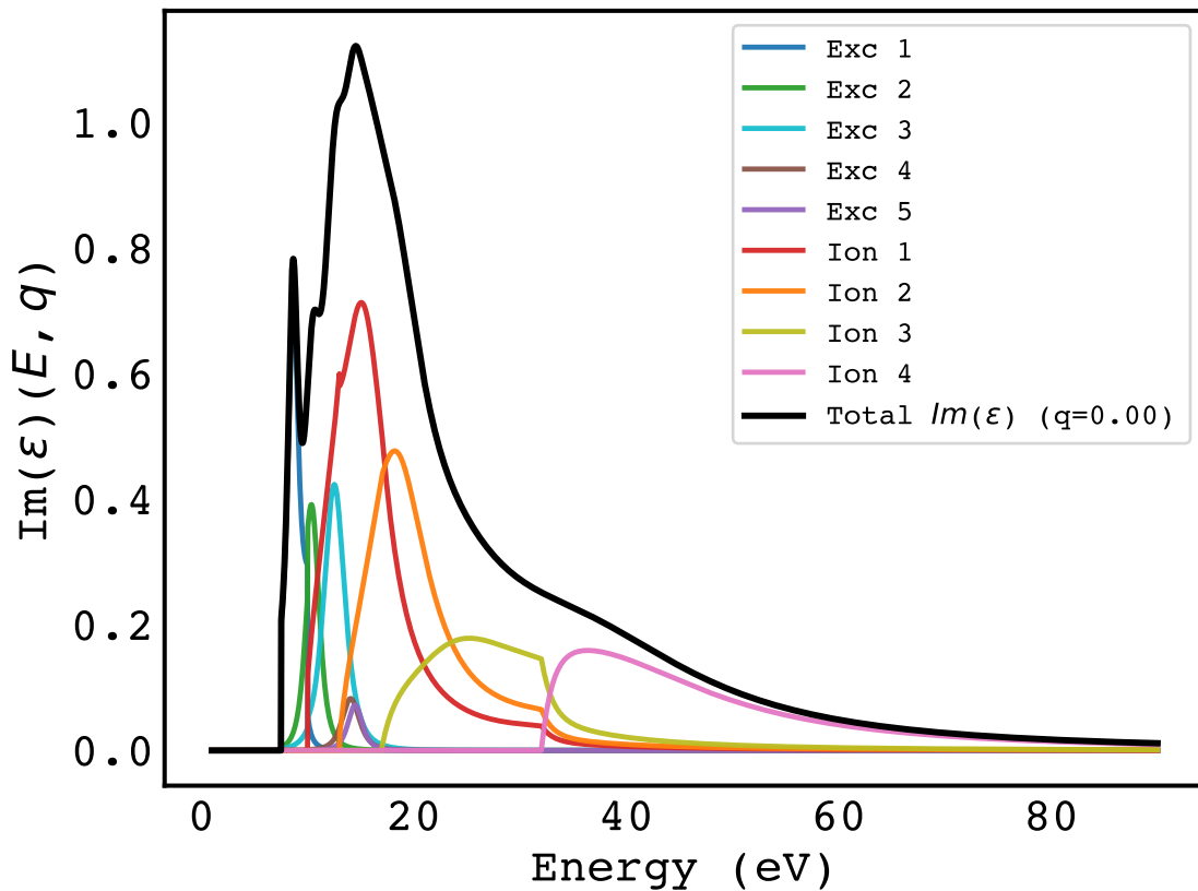
Channel-resolved \text{Im}(\epsilon) at q = 0.00 ; amorphous ice
