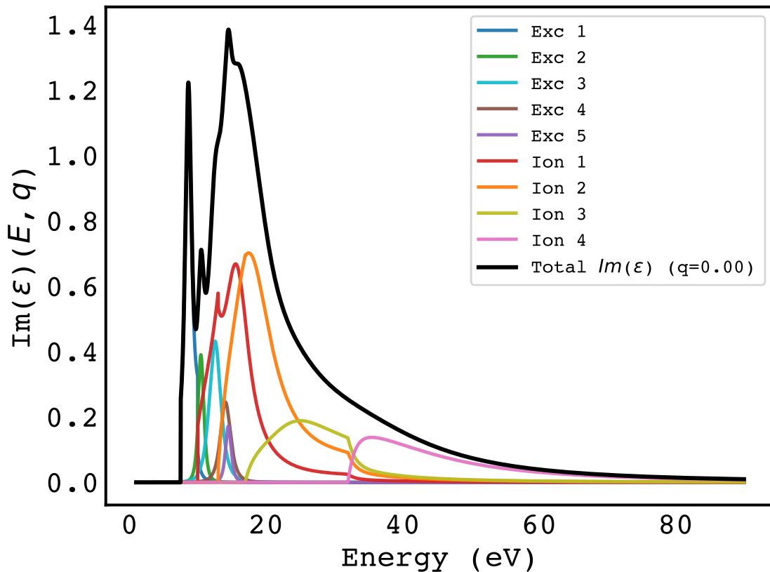
Channel-resolved \text{Im}(\varepsilon) at q = 0.00 ; hexagonal ice
