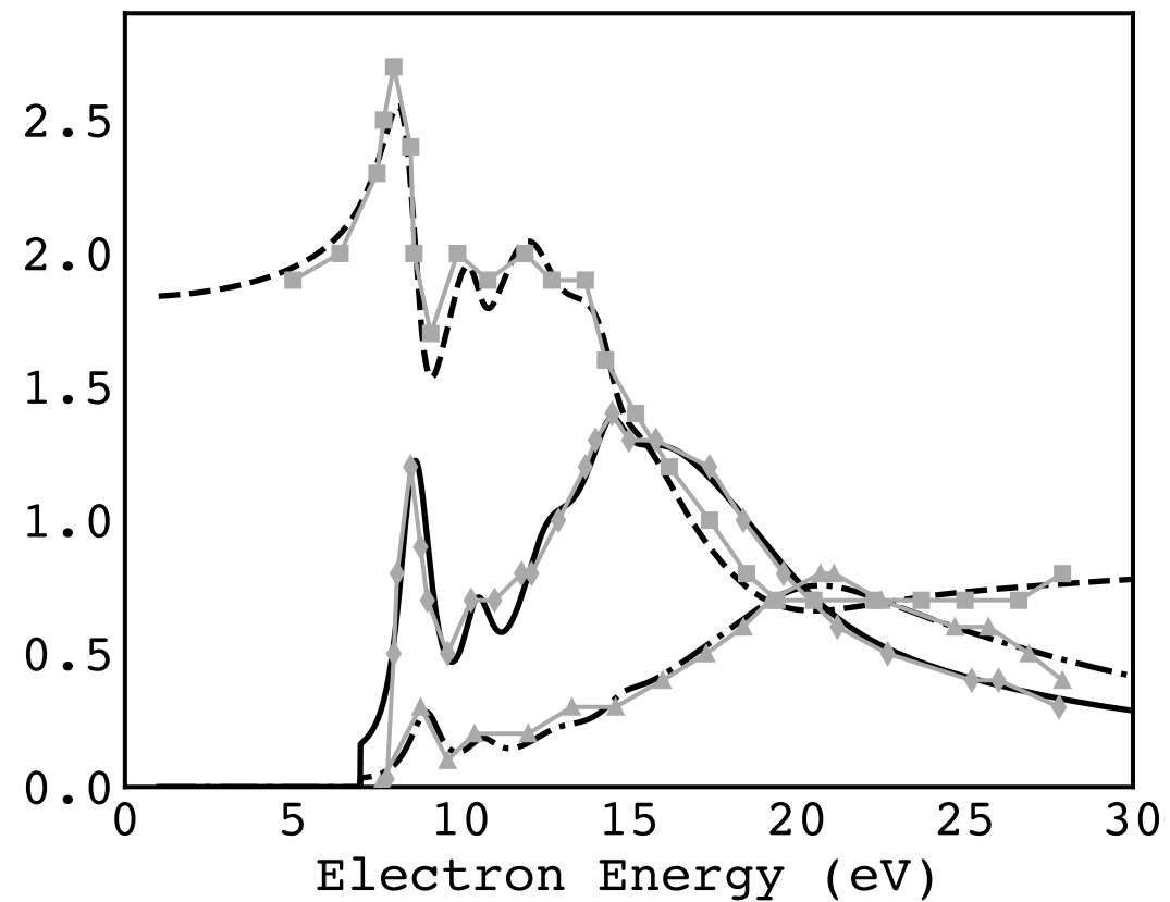
Hexagonal Ice
