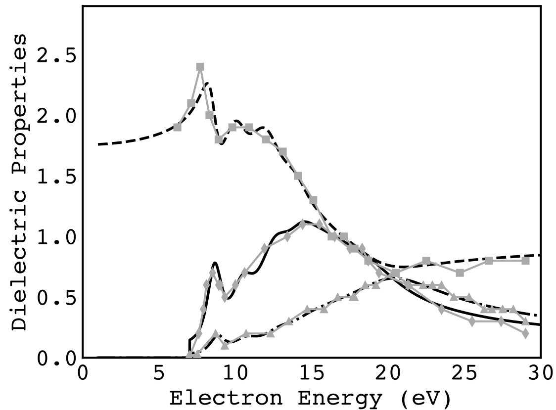
Amorphous Ice
