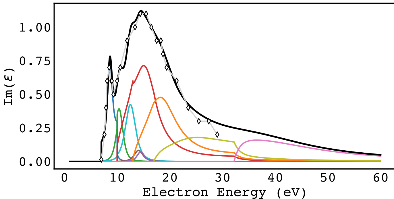
Channel-resolved \text{Im}(\varepsilon) at q = 0.0 ; amorphous ice
