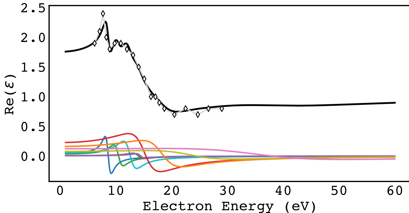
Channel-resolved \text{Re}(\varepsilon) at q = 0.0 ; amorphous ice
