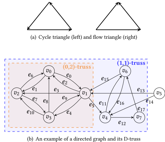
Figure 1: Illustrations of directed triangles and D-truss.
